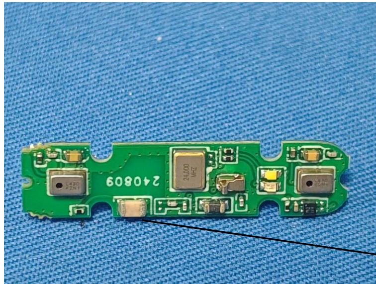
Ceramic antenna
