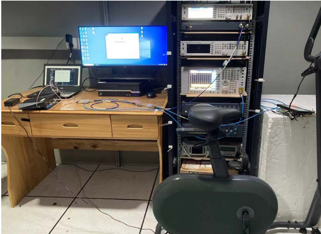
ANTENNA-PORT CONDUCTED
