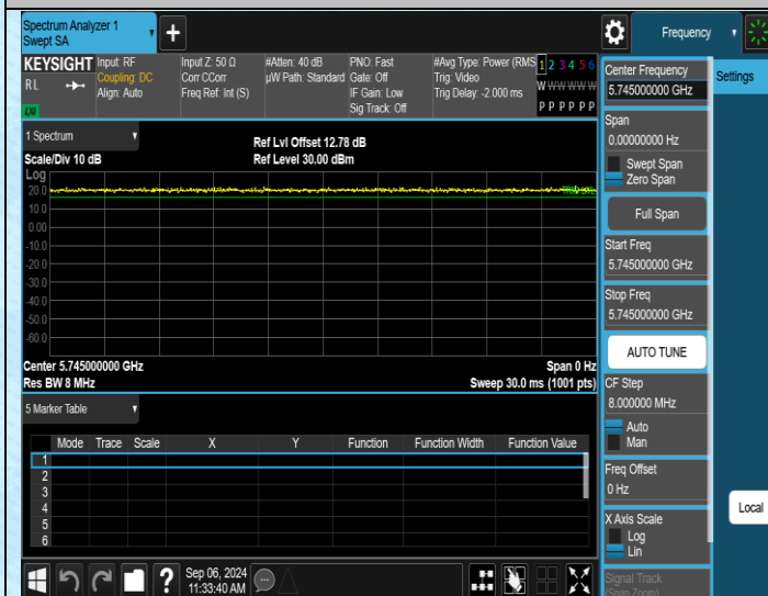
NTNV-11AC20SISO-Ant3-5745
