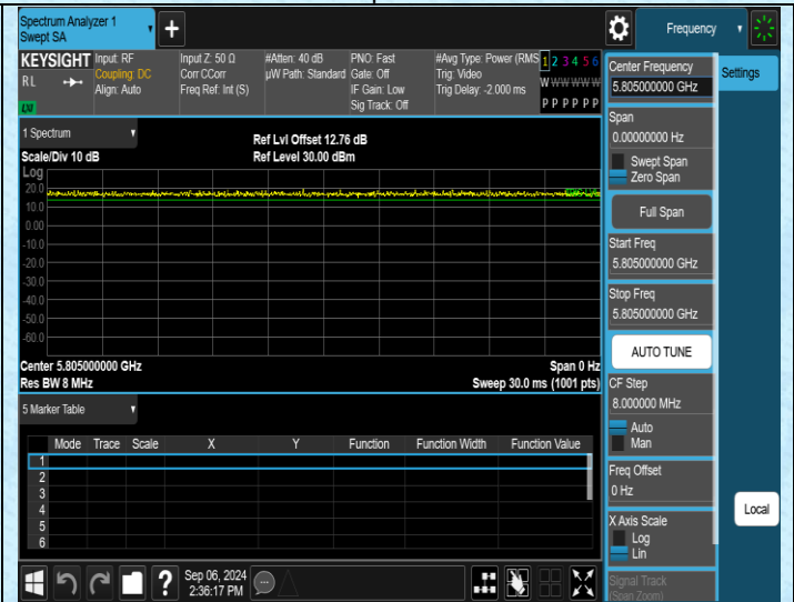
NTNV-11AC20MIMO-Ant4-5805
