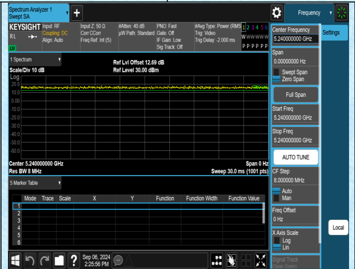
NTNV-11AC20MIMO-Ant4-5240
