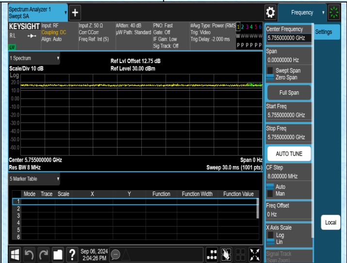
NTNV-11AC40SISO-Ant4-5755
