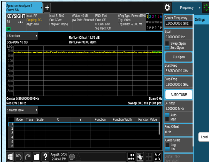
NTNV-11AC20MIMO-Ant3-5805
