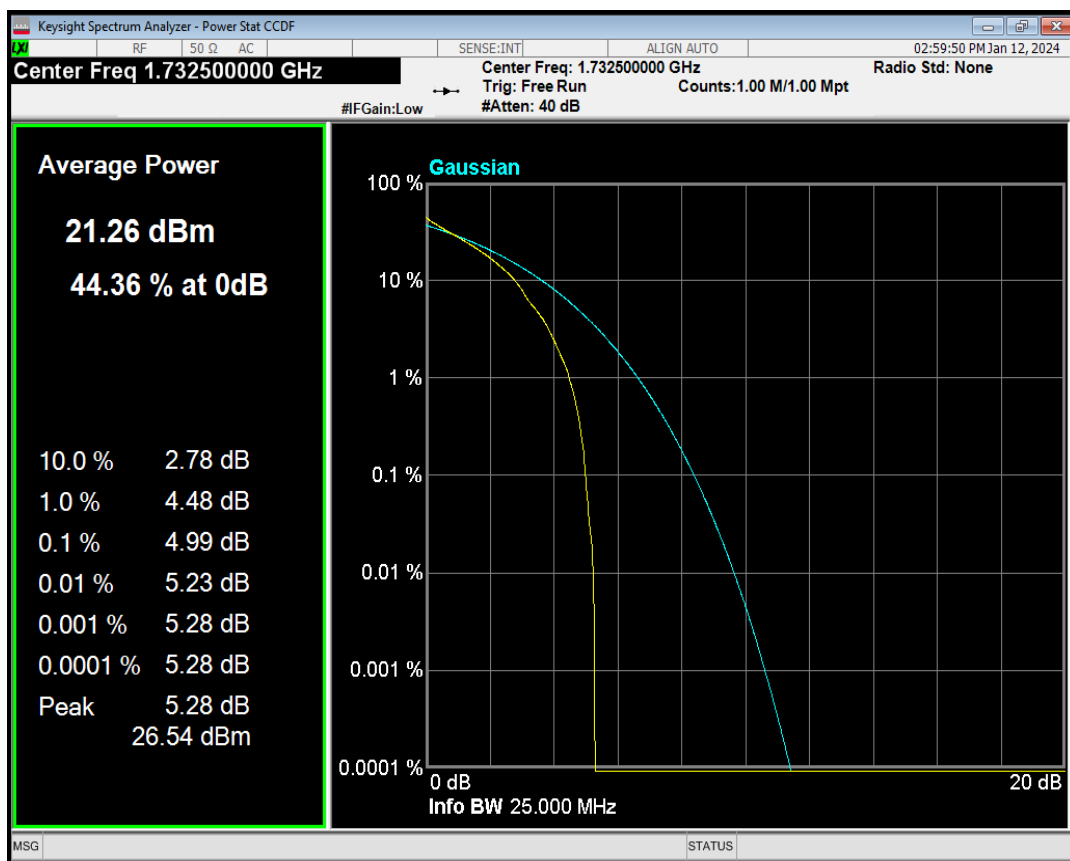
Band4 QPSK BW=5MHz Channel=20175 RB Size=1 Position=#Max
