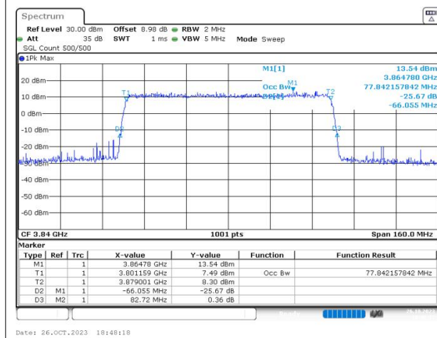
n77(3700-3980) SCS=30kHz CP_QAM64 BW=80MHz Channel=656000 RB=217@0
