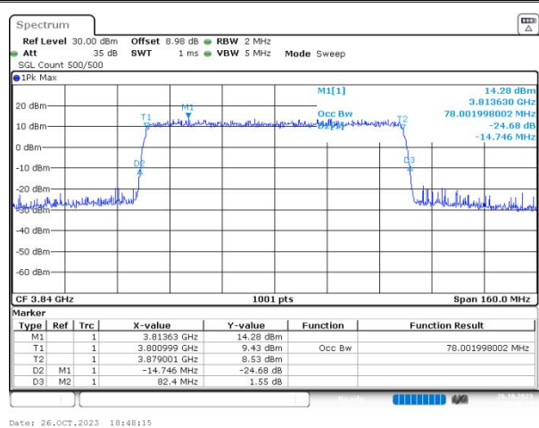
n77(3700-3980) SCS=30kHz CP_QAM16 BW=80MHz Channel=656000 RB=217@0
