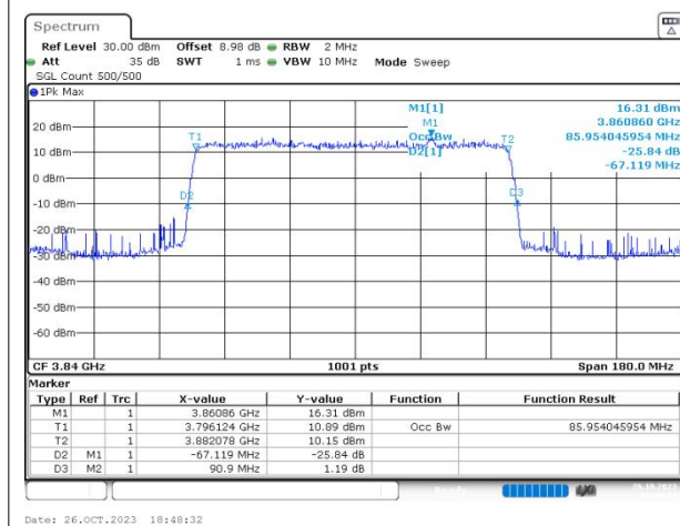
n77(3700-3980) SCS=30kHz DFT_BPSK BW=90MHz Channel=656000 RB=240@0
