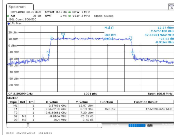
n41 SCS=30kHz CP_QAM64 BW=50MHz Channel=518598 RB=133@0
