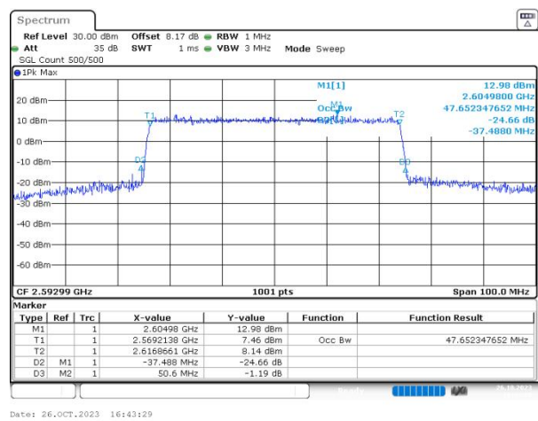
n41 SCS=30kHz CP_QAM16 BW=50MHz Channel=518598 RB=133@0
