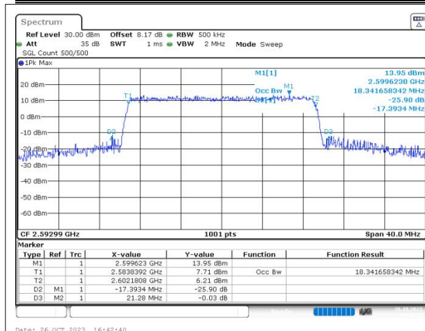
n41 SCS=30kHz CP_QAM16 BW=20MHz Channel=518598 RB=51@0
