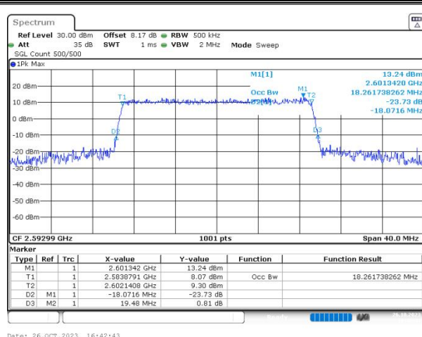
n41 SCS=30kHz CP_QAM64 BW=20MHz Channel=518598 RB=51@0
