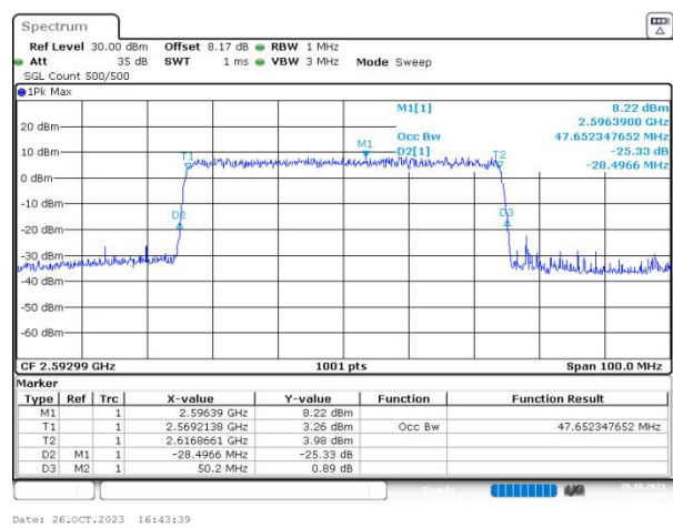
n41 SCS=30kHz CP_QAM256 BW=50MHz Channel=518598 RB=133@0
