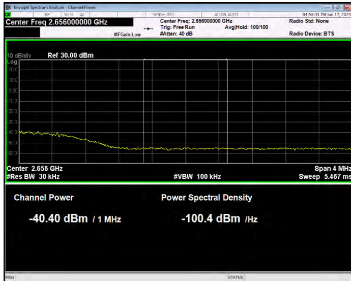
Band41(2555-2655) 16QAM BW=15MHz Channel=41165 RB Size=1 Position=#0 Normal
