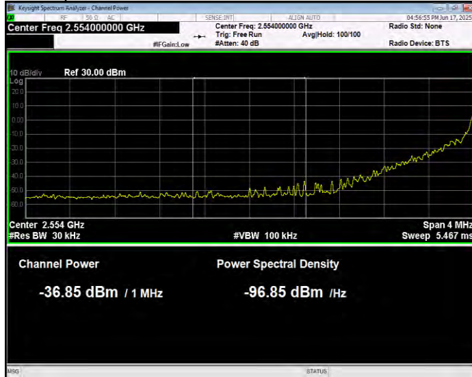
Band41(2555-2655) 16QAM BW=20MHz Channel=40340 RB Size=1 Position=#0 Normal
