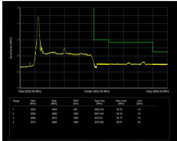
Band41(2555-2655) QPSK BW=5MHz Channel=40265 RB Size=1 Position=#0 Extended
