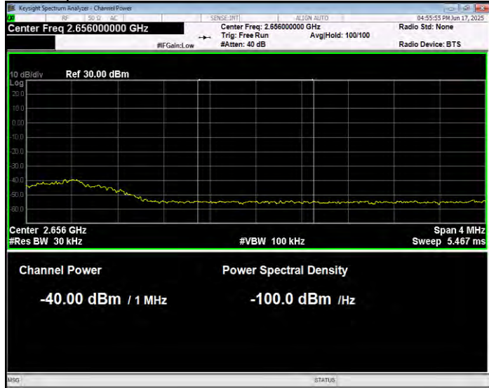
Band41(2555-2655) 16QAM BW=10MHz Channel=41190 RB Size=1 Position=#0 Normal
