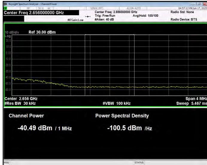
Band41(2555-2655) 16QAM BW=20MHz Channel=41140 RB Size=1 Position=#0 Normal
