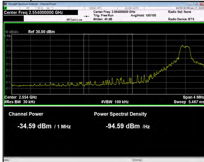
Band41(2555-2655) QPSK BW=10MHz Channel=40290 RB Size=1 Position=#0 Normal
