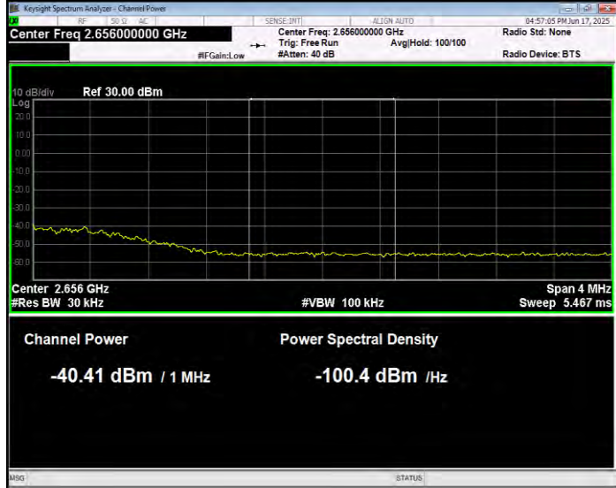
Band41(2555-2655) QPSK BW=20MHz Channel=41140 RB Size=1 Position=#0 Normal
