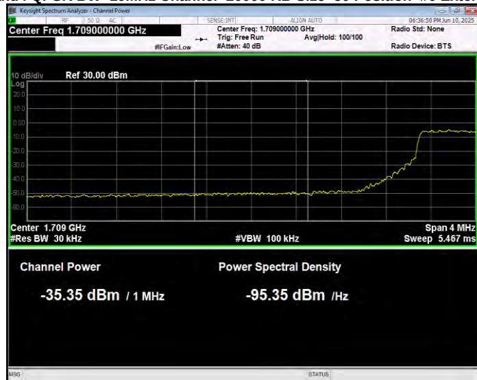
Band4 QPSK BW=10MHz Channel=20000 RB Size=50 Position=#0 Normal
