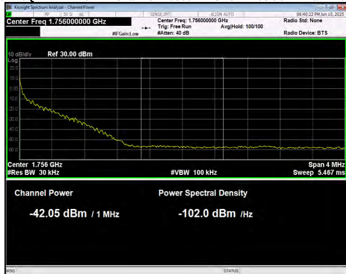
Band4 16QAM BW=20MHz Channel=20300 RB Size=1 Position=#Max Normal
