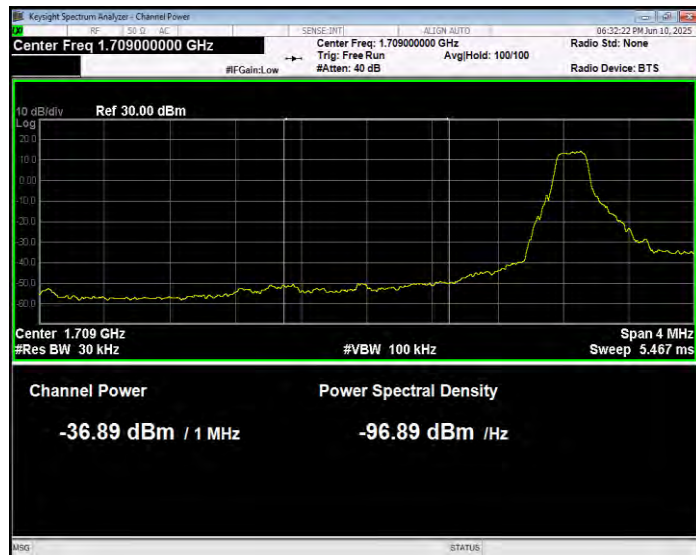
Band4 QPSK BW=1.4MHz Channel=19957 RB Size=1 Position=#0 Normal
