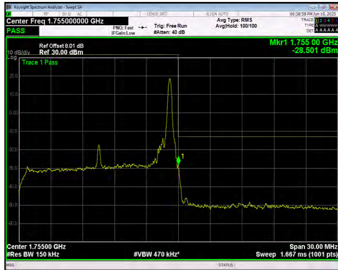
Band4 16QAM BW=15MHz Channel=20325 RB Size=75 Position=#0 Extended
