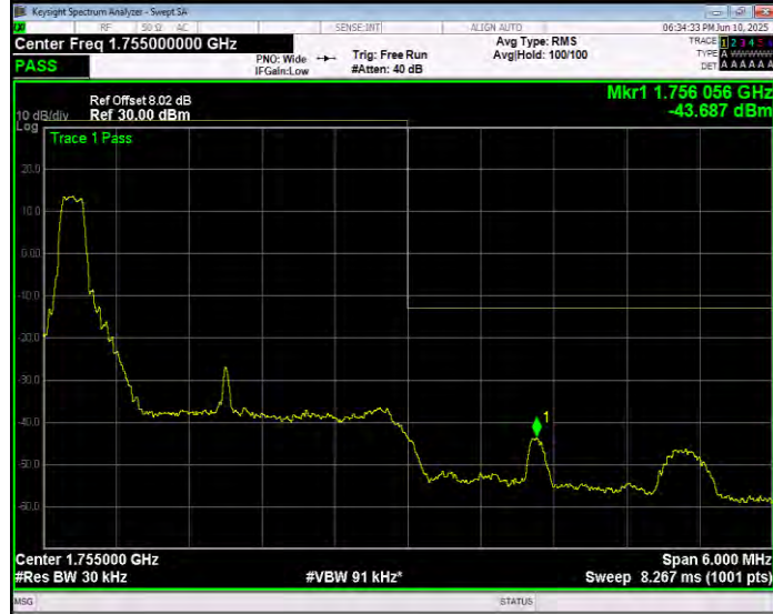
Band4 QPSK BW=3MHz Channel=20385 RB Size=1 Position=#Max Extended
