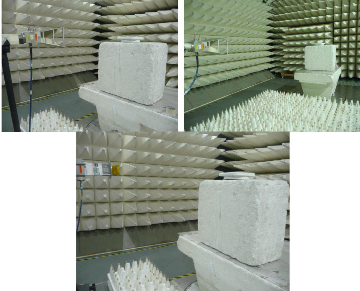
Photograph No.4 Spurious and band edge emissions measurement setup in the anechoic chamber above 1 GHz
