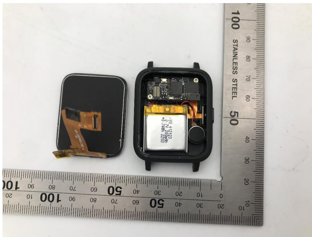
Photo 1 Inside of EUT
