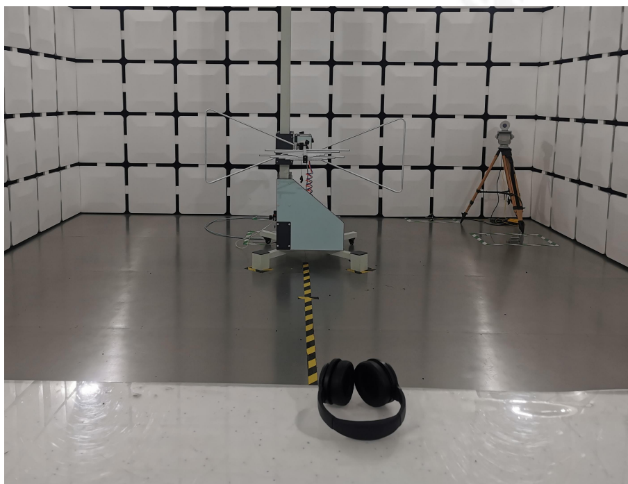
Radiated Emission
