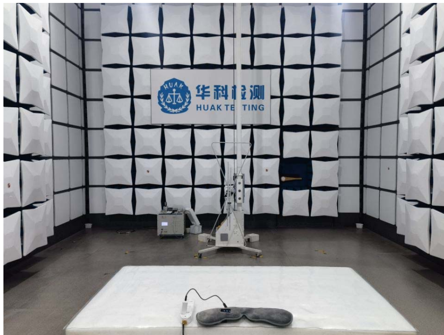
Model: BTEM-03 Radiated Emissions
