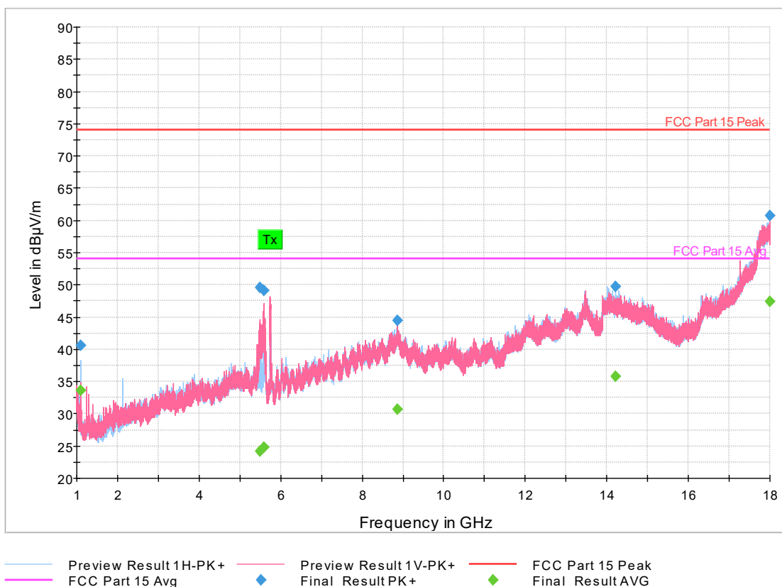
Figure 92: 1-18 GHz 802.11ax Mode 20 MHz, Low Channel
