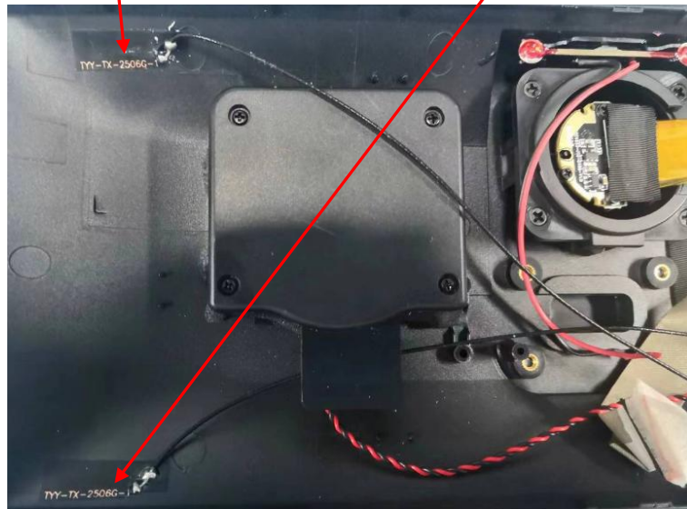
BT PCB Antenna
