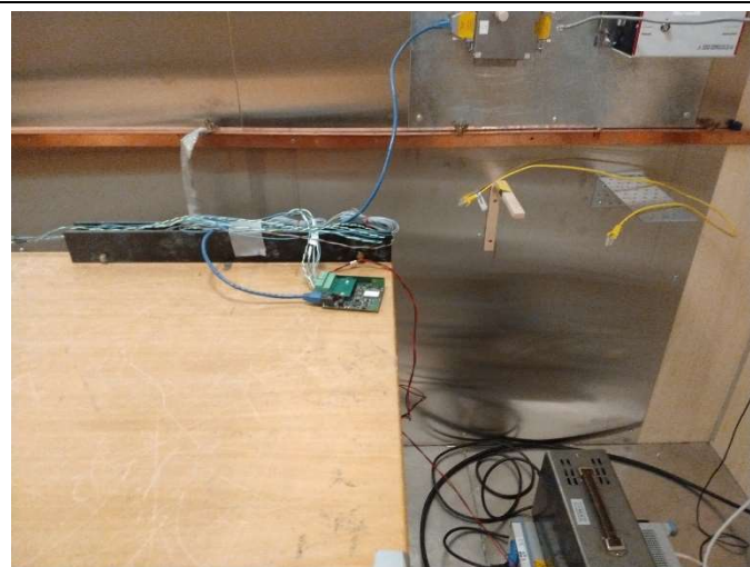
Conducted Emission
