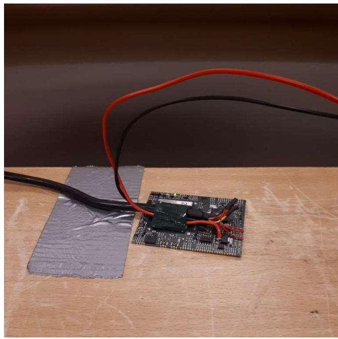
Conducted Emission Card C, the USB-cable is temporary and was used for monitoring only
