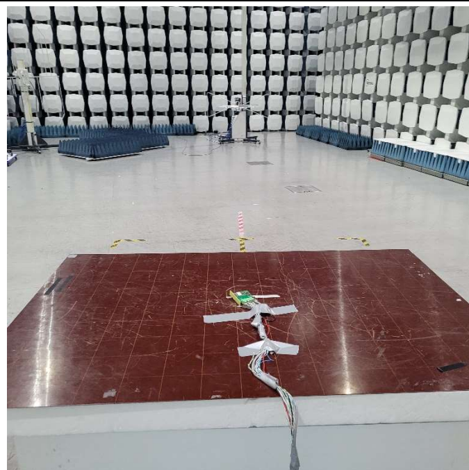
Radiated Emission < 1 GHz
