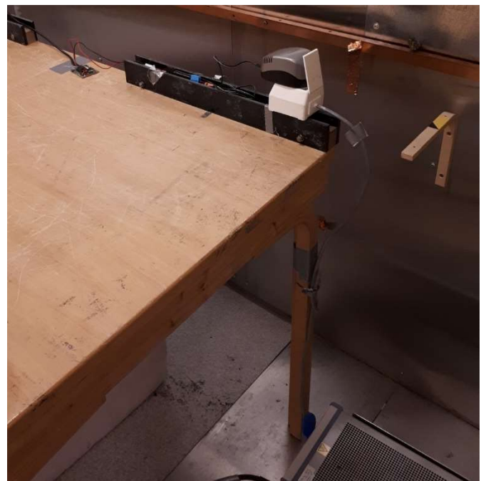
Conducted Emission Card C, ACDC-converter to the left
