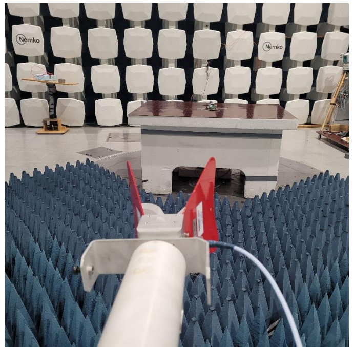
Radiated Emission > 1 GHz
