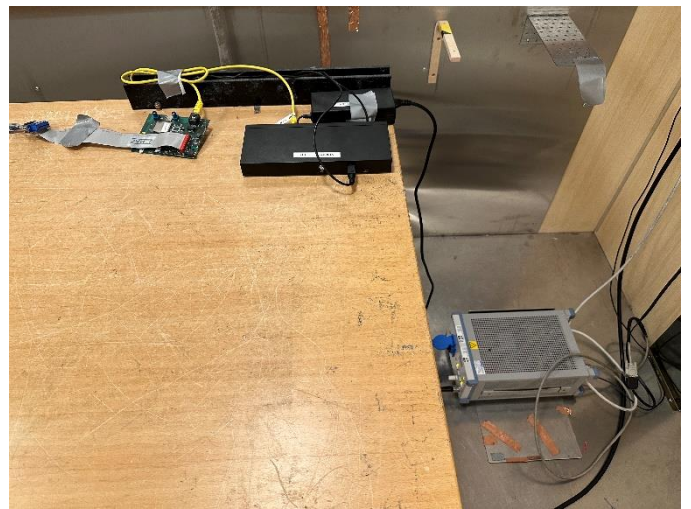
Conducted Emission
