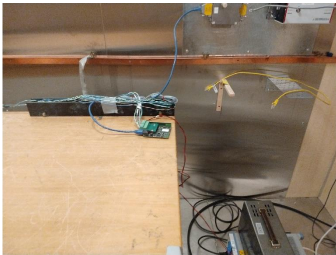
Conducted Emission
