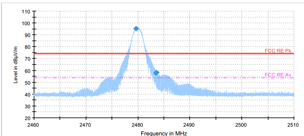
BLE 1Mbps, Highest Channel (2 480 MHz)_Peak
