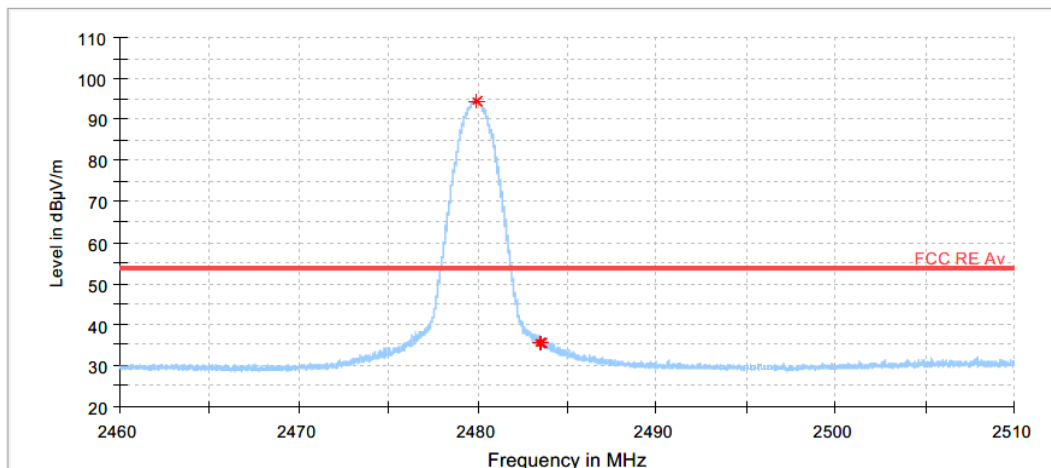
BLE 1Mbps, Highest Channel (2 480 MHz)_Average
