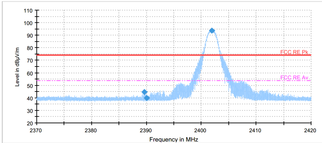
BLE 1Mbps, Lowest Channel (2 402 MHz)_Peak
