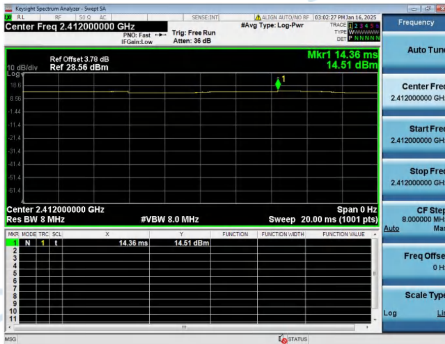
Duty_Cycle_NVNT_ANT1_802_11b_2412
