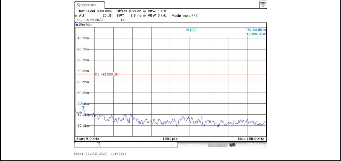
Band4-1412-2-0.009~0.15MHz
