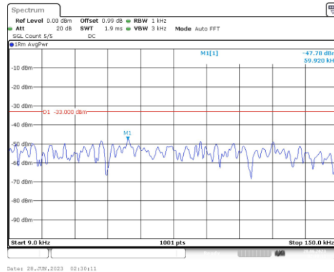
Band12-3MHz-QPSK-23165-1RB#0-Range1:0.009~0.15MHz
