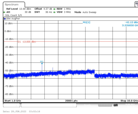
Band12-5MHz-QPSK-23095-1RB#0-Range4:1000~10000MHz
