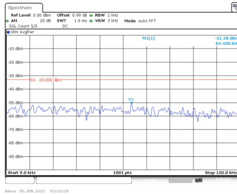
Band12-5MHz-16QAM-23095-1RB#0-Range1:0.009~0.15MHz
