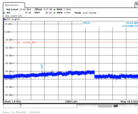
Band12-3MHz-16QAM-23095-1RB#0-Range4:1000~10000MHz
