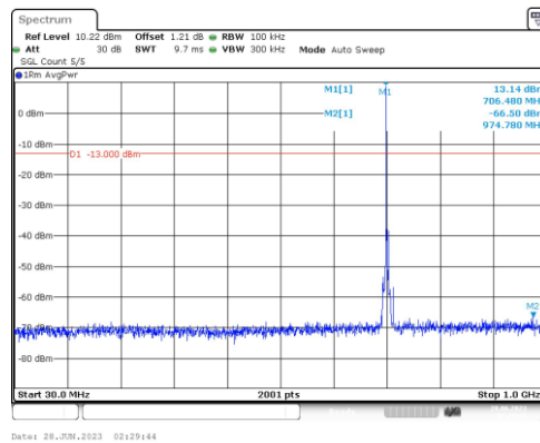
Band12-3MHz-16QAM-23095-1RB#0-Range3:30~1000MHz
