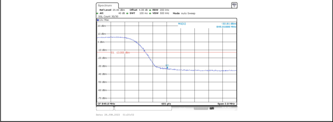
Band5-10MHz-QPSK-20600-50RB#0
