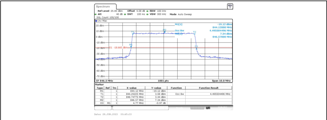
Band5-5MHz-16QAM-20625-25RB#0-4.496
