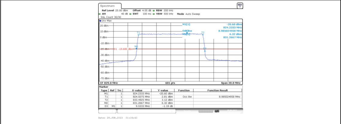
Band5-10MHz-QPSK-20450-50RB#0-8.985
