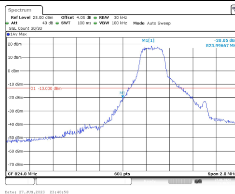
Band5-1.4MHz-QPSK-20407-1RB#0
