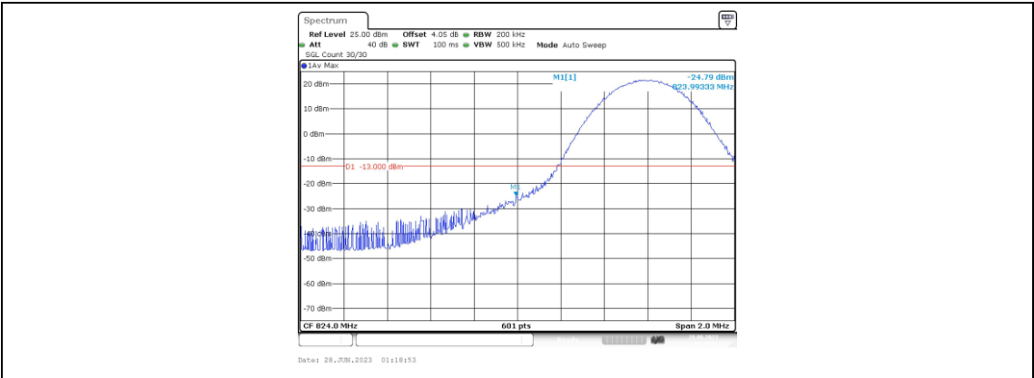
Band5-10MHz-16QAM-20450-1RB#0
