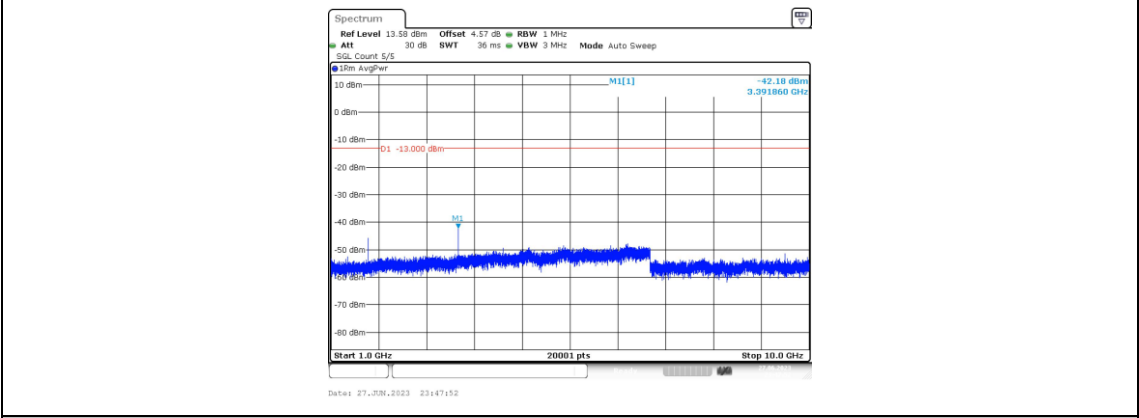
Band5-1.4MHz-QPSK-20643-1RB#0-Range4:1000~10000MHz
