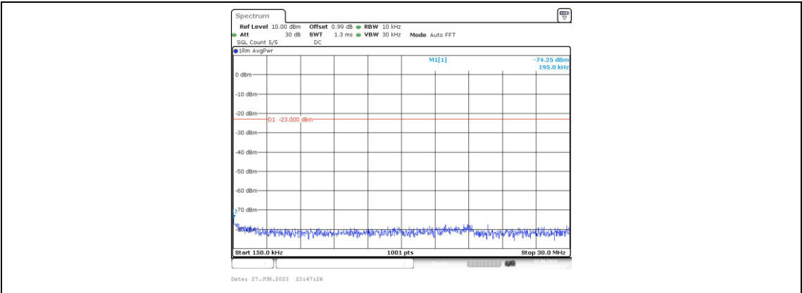
Band5-1.4MHz-QPSK-20643-1RB#0-Range2:0.15~30MHz
