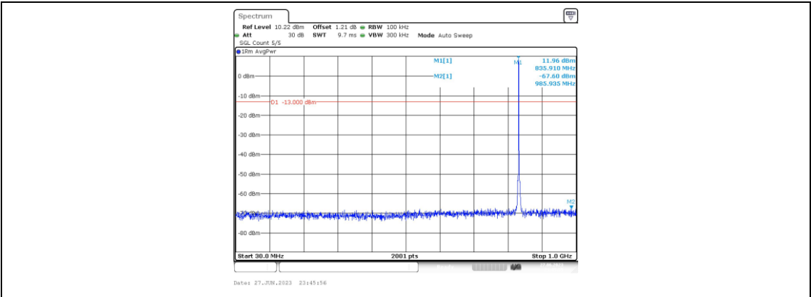
Band5-1.4MHz-QPSK-20525-1RB#0-Range3:30~1000MHz
