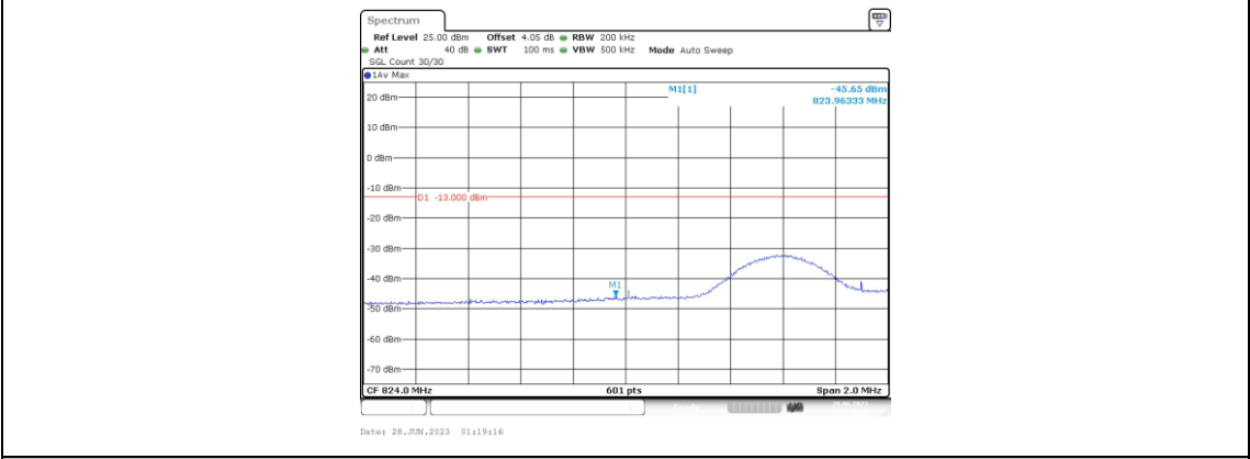
Band5-10MHz-16QAM-20450-1RB#49
