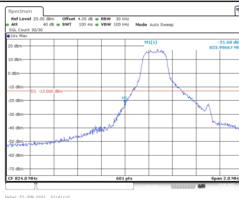
Band5-1.4MHz-16QAM-20407-1RB#0
