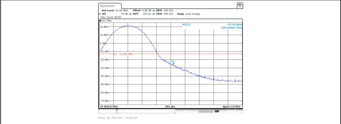
Band5-10MHz-16QAM-20600-1RB#49
