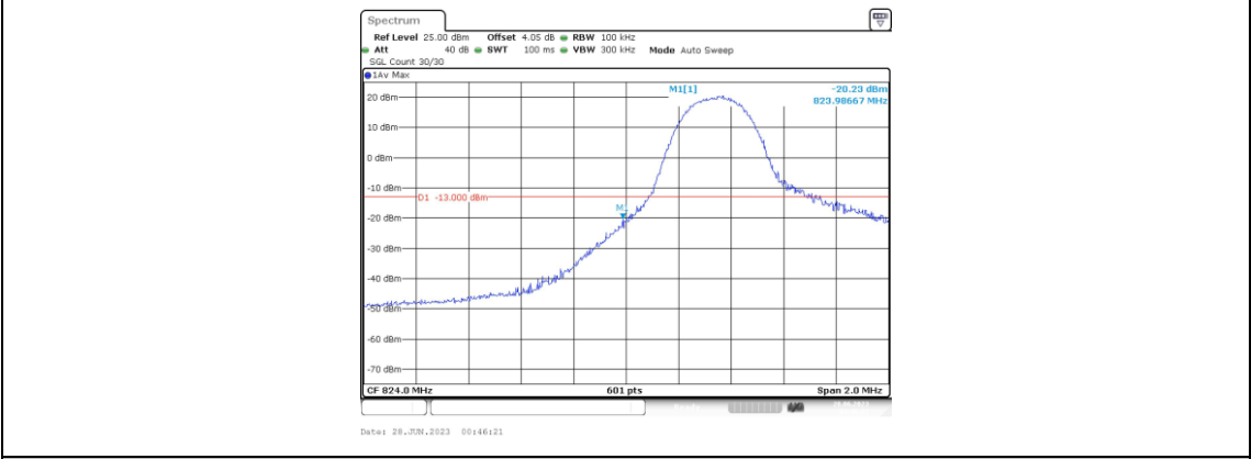
Band5-5MHz-16QAM-20425-1RB#0
