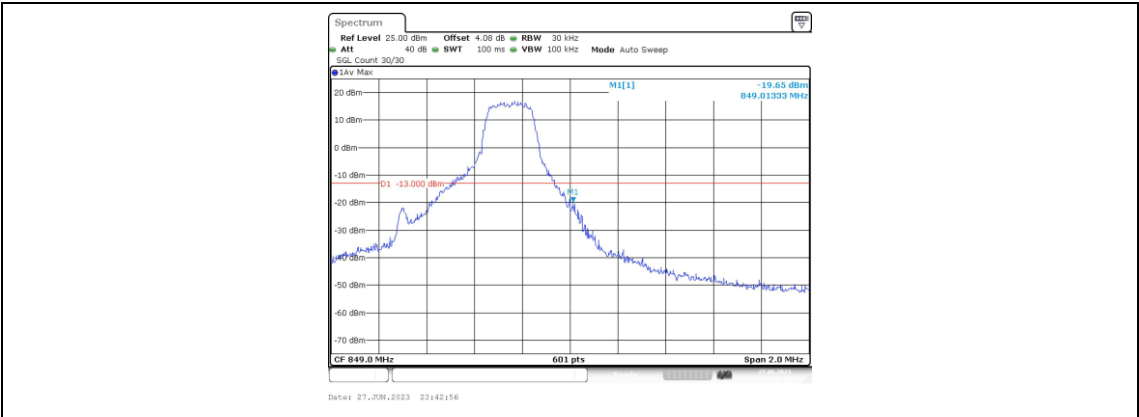
Band5-1.4MHz-16QAM-20643-1RB#5
