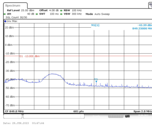
Band5-5MHz-16QAM-20625-1RB#0
