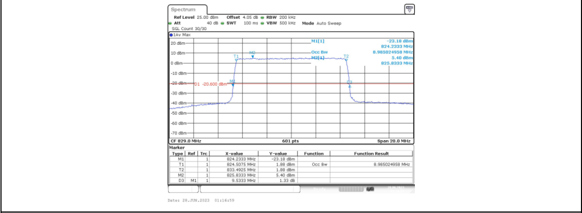
Band5-10MHz-16QAM-20450-50RB#0-8.985
