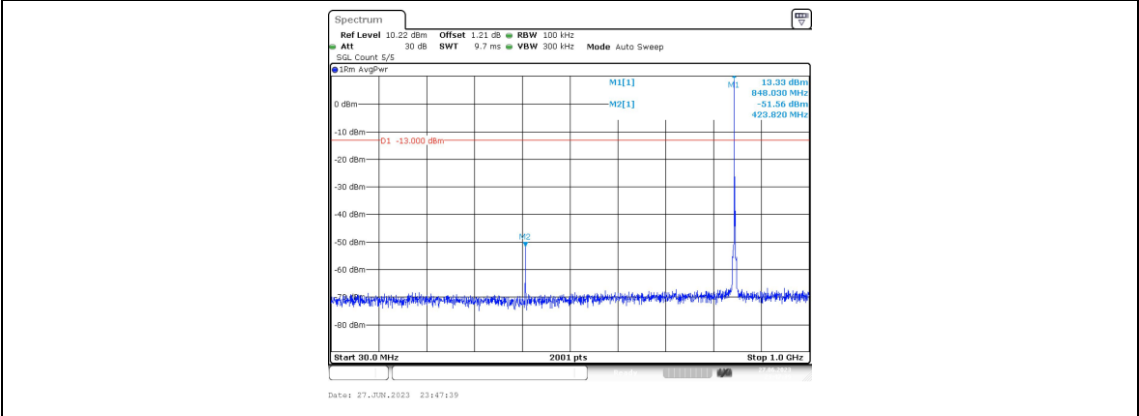
Band5-1.4MHz-QPSK-20643-1RB#0-Range3:30~1000MHz
