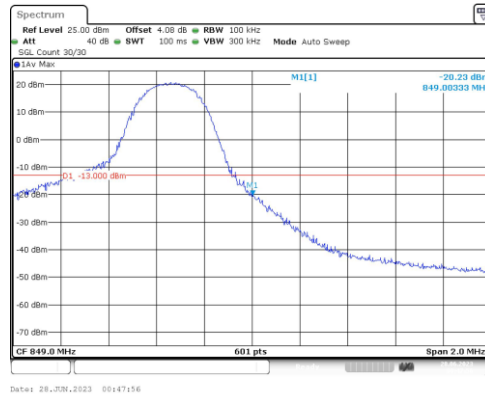
Band5-5MHz-QPSK-20625-1RB#24
