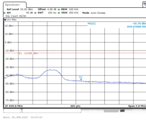
Band5-5MHz-QPSK-20625-1RB#0
