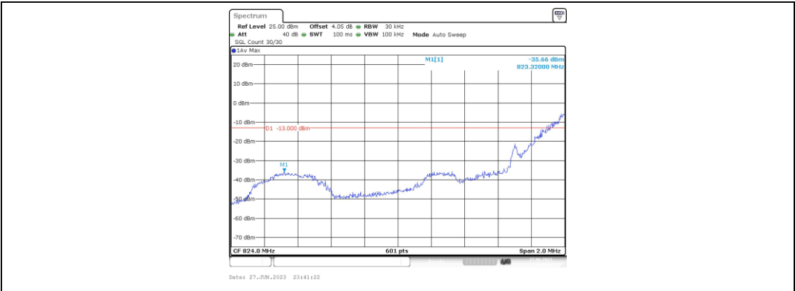
Band5-1.4MHz-QPSK-20407-1RB#5
