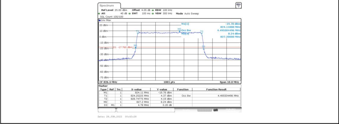
Band5-5MHz-QPSK-20425-25RB#0-4.496
