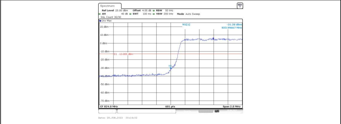
Band5-3MHz-16QAM-20415-15RB#0
