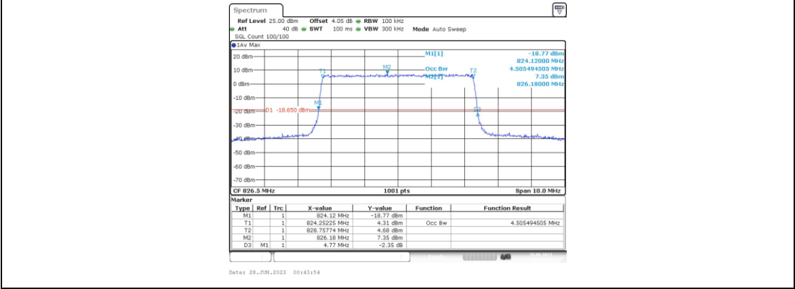
Band5-5MHz-QPSK-20425-25RB#0-4.496
