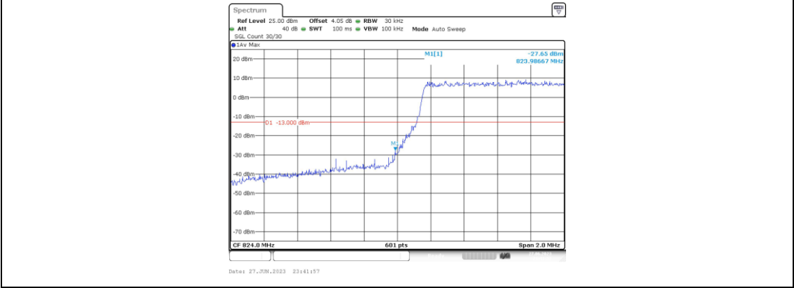
Band5-1.4MHz-QPSK-20407-6RB#0
