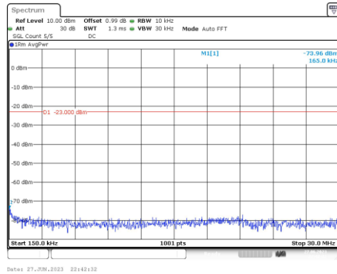
Band4-15MHz-16QAM-20325-1RB#0-Range2:0.15~30MHz
