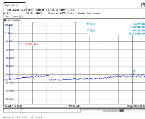
Band4-3MHz-16QAM-20175-1RB#0-Range4:1000~20000MHz
