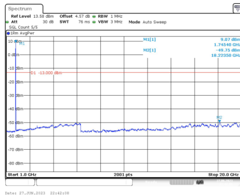
Band4-15MHz-QPSK-20325-1RB#0-Range4:1000~20000MHz
