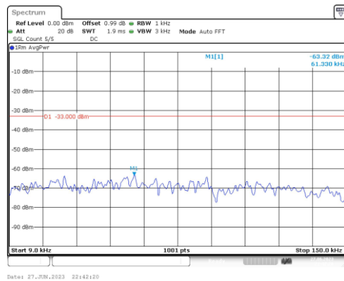
Band4-15MHz-16QAM-20325-1RB#0-Range1:0.009~0.15MHz
