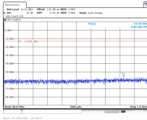
Band4-10MHz-QPSK-20000-1RB#0-Range3:30~1000MHz
