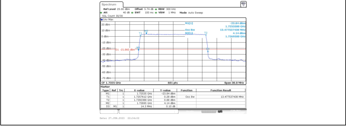
Band4-15MHz-QPSK-20175-75RB#0-13.478
