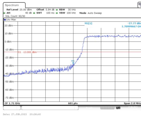
Band4-1.4MHz-QPSK-19957-6RB#0
