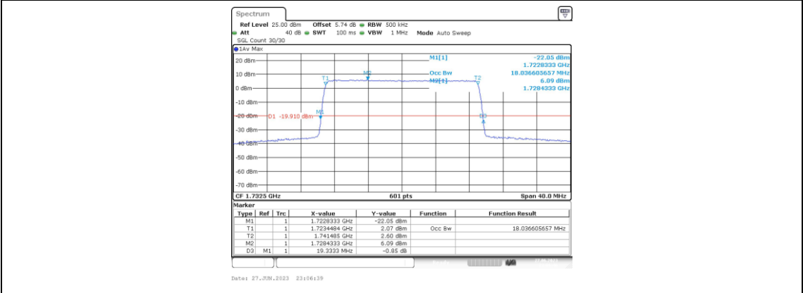
Band4-20MHz-QPSK-20175-100RB#0-18.037
