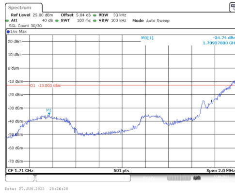
Band4-1.4MHz-16QAM-19957-1RB#5
