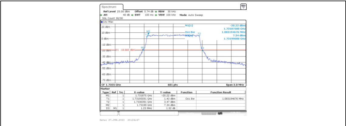
Band4-1.4MHz-16QAM-20175-6RB#0-1.083
