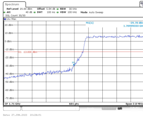
Band4-1.4MHz-16QAM-19957-6RB#0
