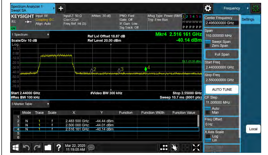
11AX20SiSO-Ant2-2462-PASS
