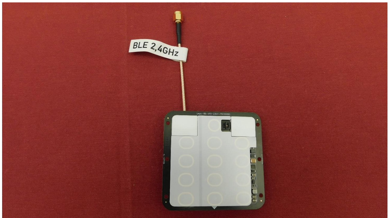
Picture 3: EUT – PBC front view with mounted keyboard
