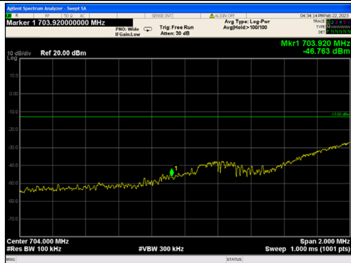
Band17_5MHz_QPSK_23755_1RB#24
