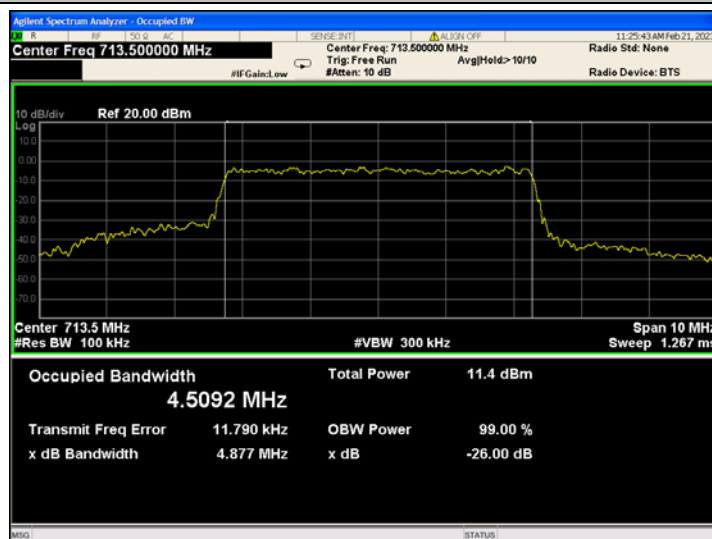
Band17_5MHz_QPSK_23825_25RB#0
