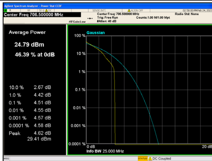
Band17_5MHz_QPSK_23755_25RB#0
