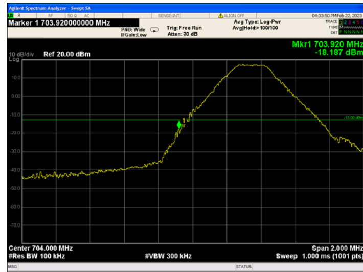
Band17_5MHz_QPSK_23755_1RB#13
