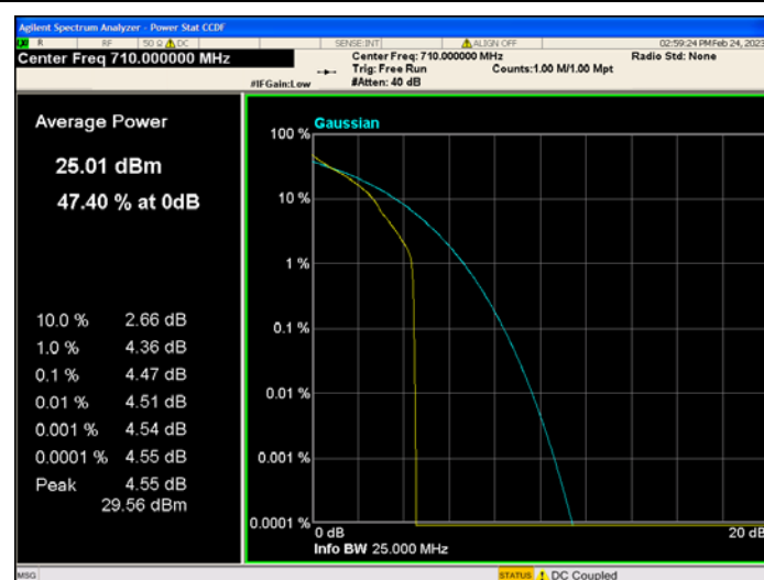
Band17_5MHz_QPSK_23790_1RB#0
