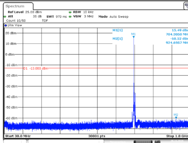
Band17_5MHz_QPSK_23755_1RB#0
