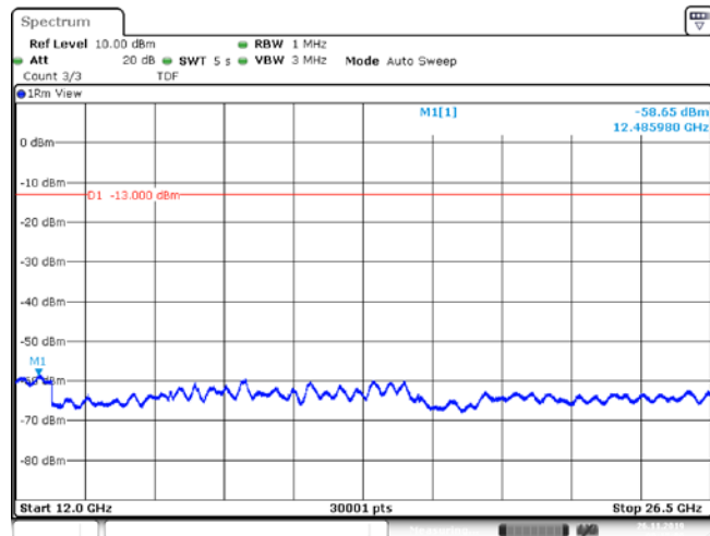
Band5_3MHz_QPSK_20415_1RB#14
