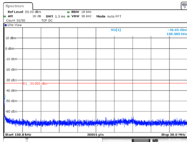
Band5_3MHz_16QAM_20525_1RB#14
