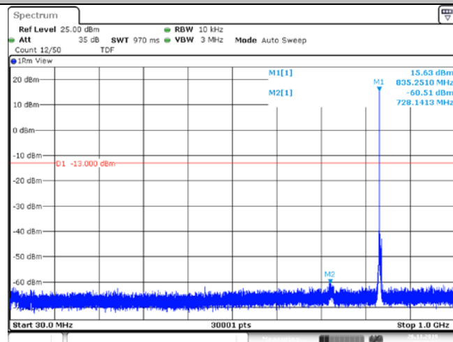
Band5_3MHz_16QAM_20525_1RB#14
