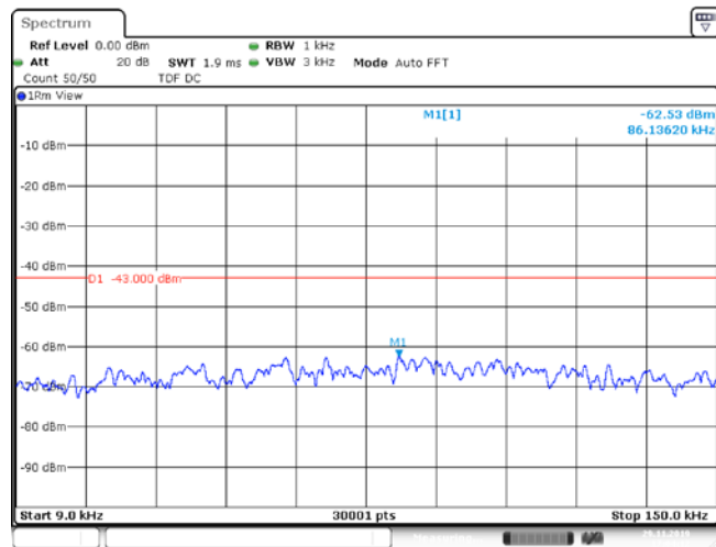
Band5_1.4MHz_QPSK_20407_3RB#3
