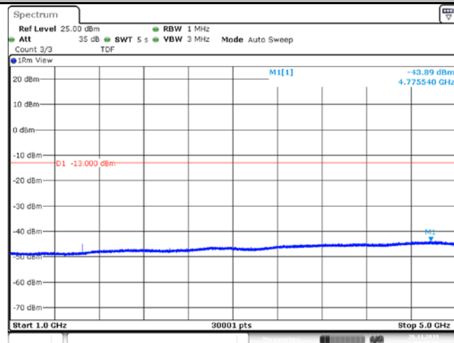
Band5_1.4MHz_QPSK_20407_3RB#3
