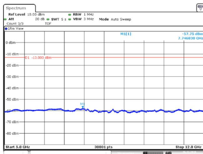
Band5_1.4MHz_QPSK_20407_3RB#3
