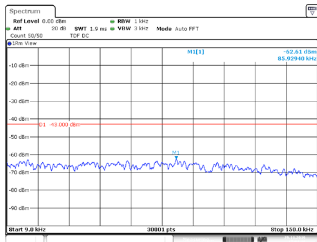
Band5_1.4MHz_16QAM_20407_1RB#2
