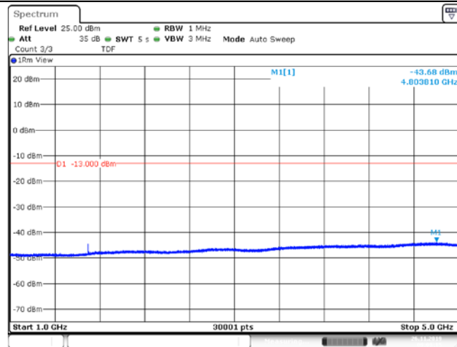
Band5_1.4MHz_16QAM_20643_1RB#2
