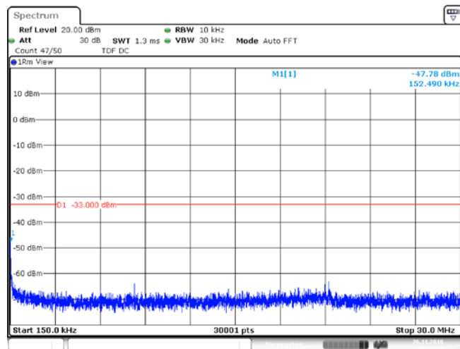
Band5_1.4MHz_QPSK_20407_3RB#3
