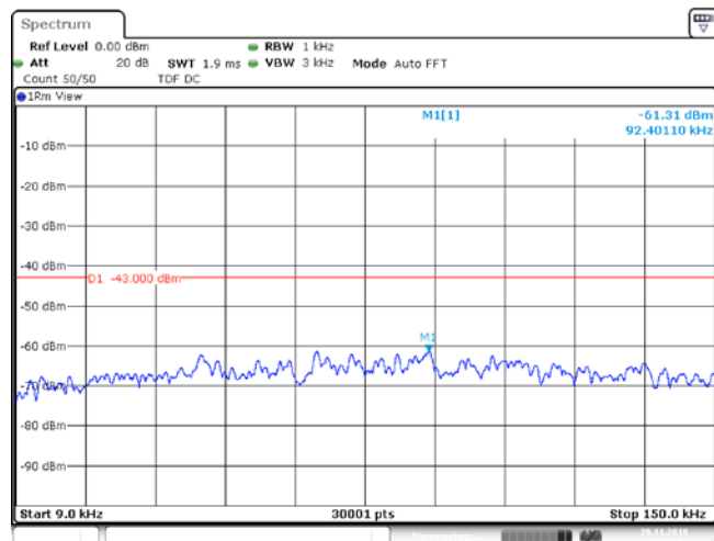
Band5_3MHz_QPSK_20525_1RB#14
