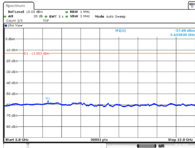
Band5_1.4MHz_QPSK_20643_3RB#3
