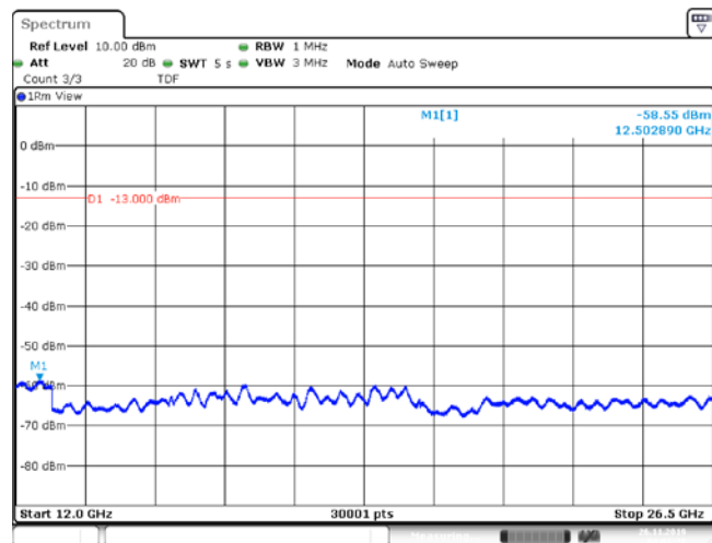
Band5_1.4MHz_QPSK_20643_3RB#3
