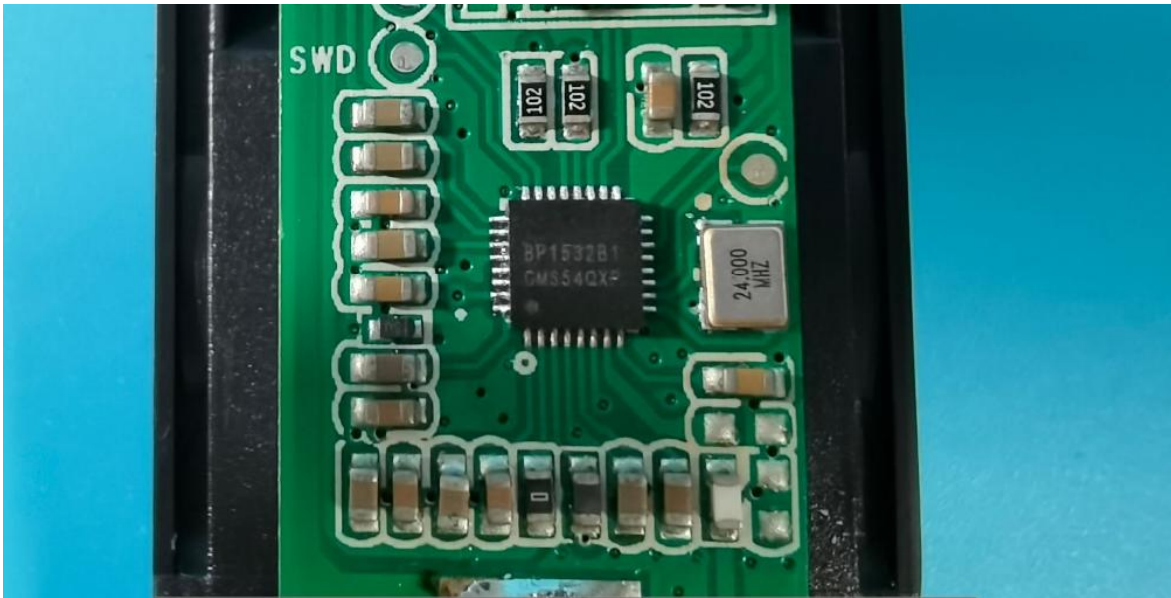
INTERNAL PHOTO OF SAMPLE PCB
