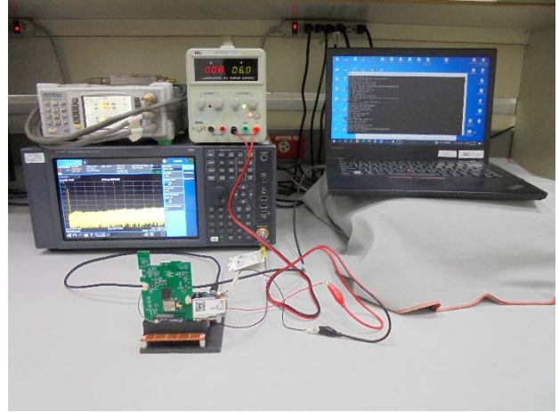
FCC_15_247_FSK_Radiated_Setup
