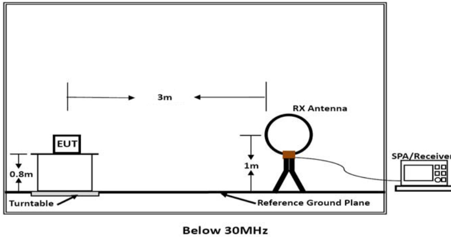
Below 30MHz
