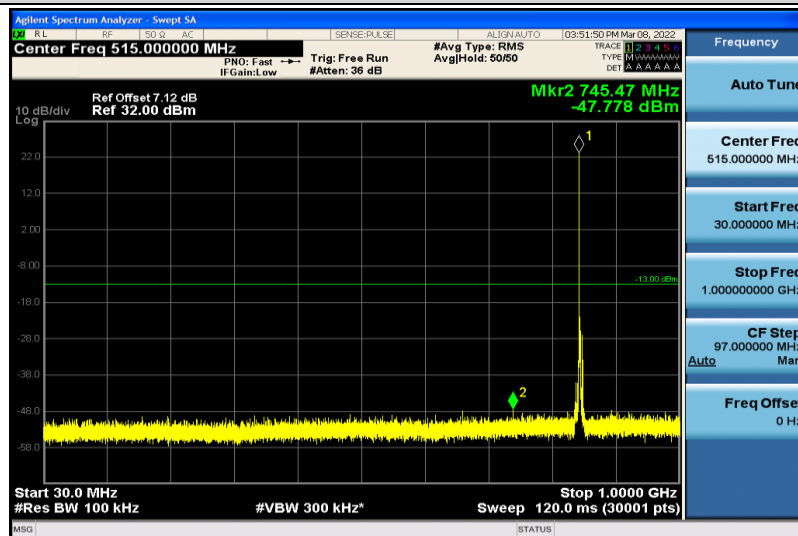
Band5-3MHz-64QAM-20635-1RB#0-30~1000MHz
