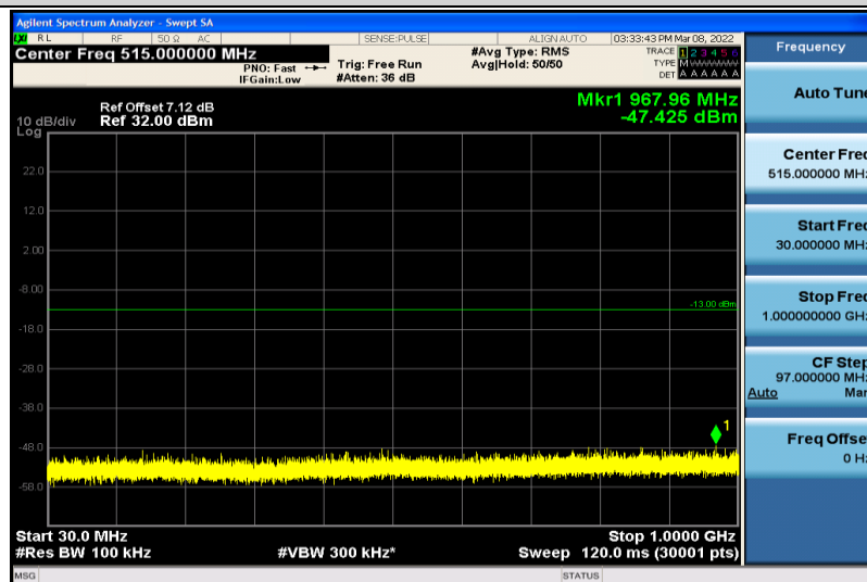
Band4-20MHz-64QAM-20175-1RB#0-30~1000MHz
