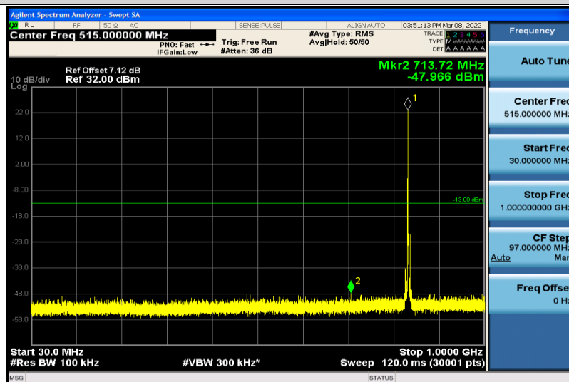
Band5-3MHz-64QAM-20525-1RB#0-30~1000MHz
