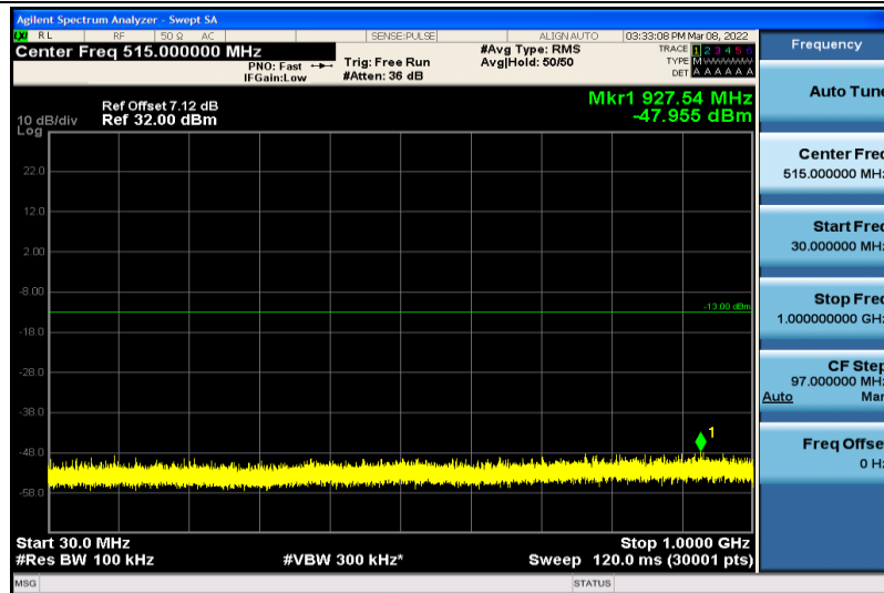
Band4-20MHz-64QAM-20050-1RB#0-30~1000MHz
