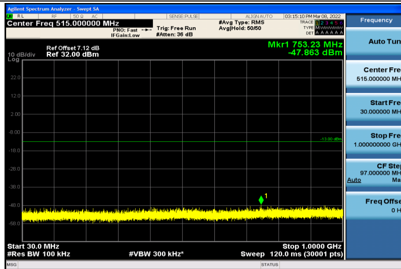
Band4-10MHz-64QAM-20000-1RB#0-30~1000MHz
