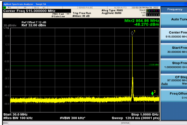
Band5-3MHz-64QAM-20415-1RB#0-30~1000MHz
