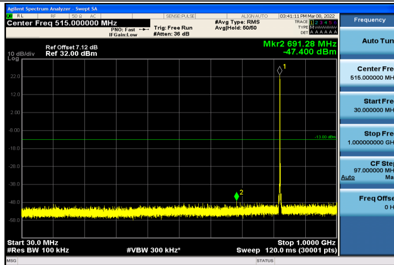
Band5-1.4MHz-64QAM-20407-1RB#0-30~1000MHz
