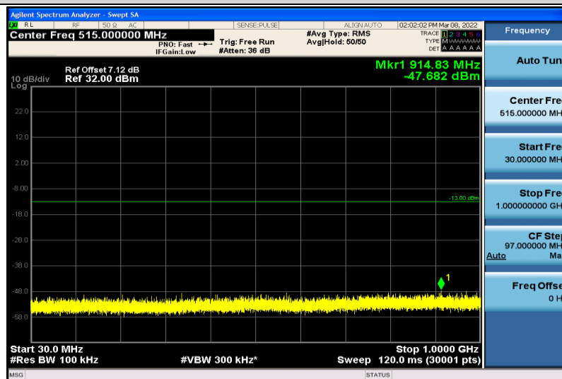
Band2-3MHz-64QAM-18900-1RB#0-30~1000MHz
