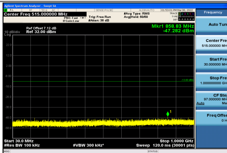
Band2-1.4MHz-64QAM-18900-1RB#0-30~1000MHz
