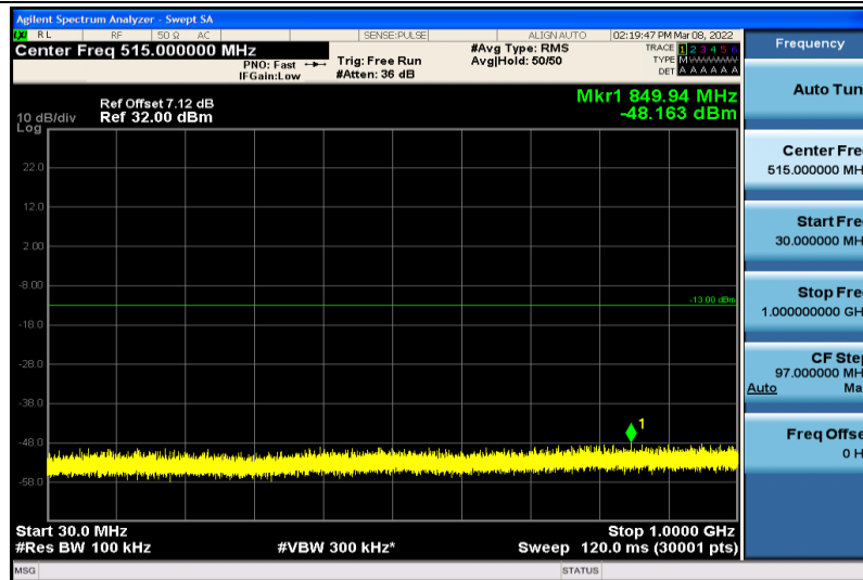
Band2-10MHz-64QAM-18650-1RB#0-30~1000MHz
