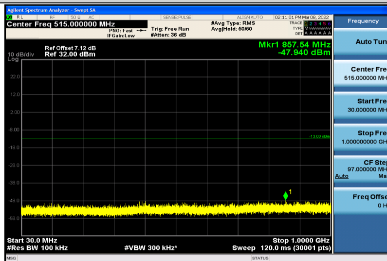
Band2-5MHz-64QAM-18900-1RB#0-30~1000MHz
