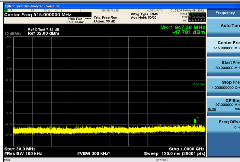
Band2-1.4MHz-64QAM-19193-1RB#0-30~1000MHz
