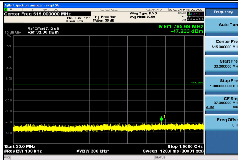
Band2-3MHz-64QAM-18615-1RB#0-30~1000MHz
