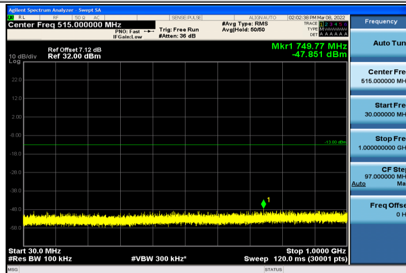
Band2-3MHz-64QAM-19185-1RB#0-30~1000MHz
