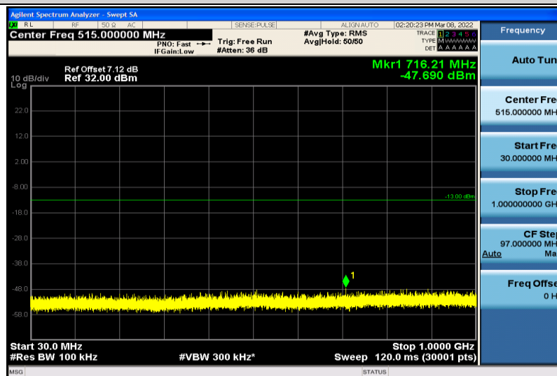
Band2-10MHz-64QAM-18900-1RB#0-30~1000MHz
