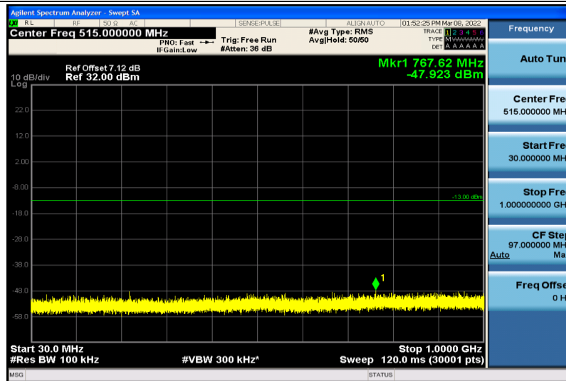
Band2-1.4MHz-64QAM-18607-1RB#0-30~1000MHz
