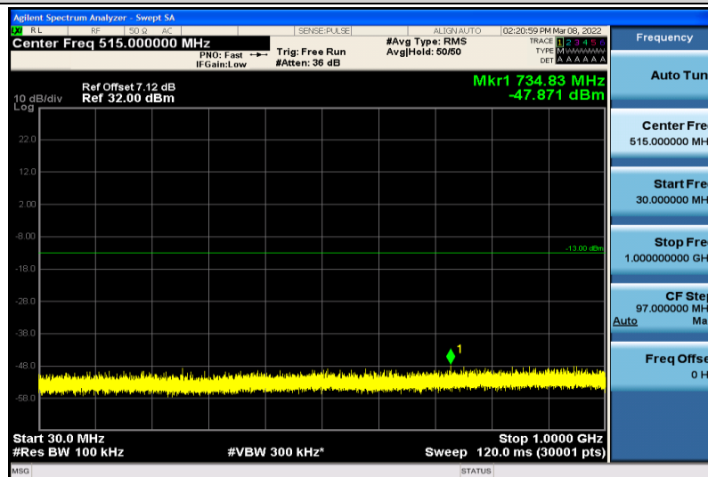
Band2-10MHz-64QAM-19150-1RB#0-30~1000MHz
