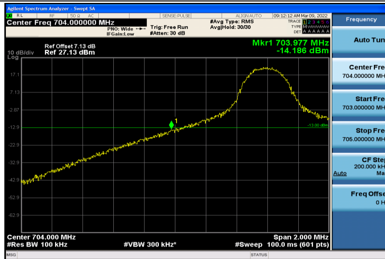
Band17-10MHz-64QAM-23780-1RB#0
