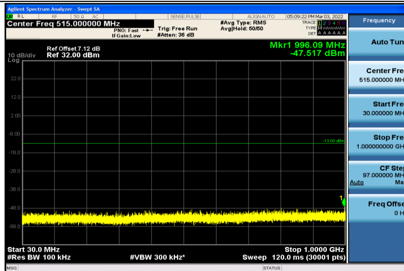
Band2-3MHz-16QAM-18900-1RB#0-30~1000MHz
