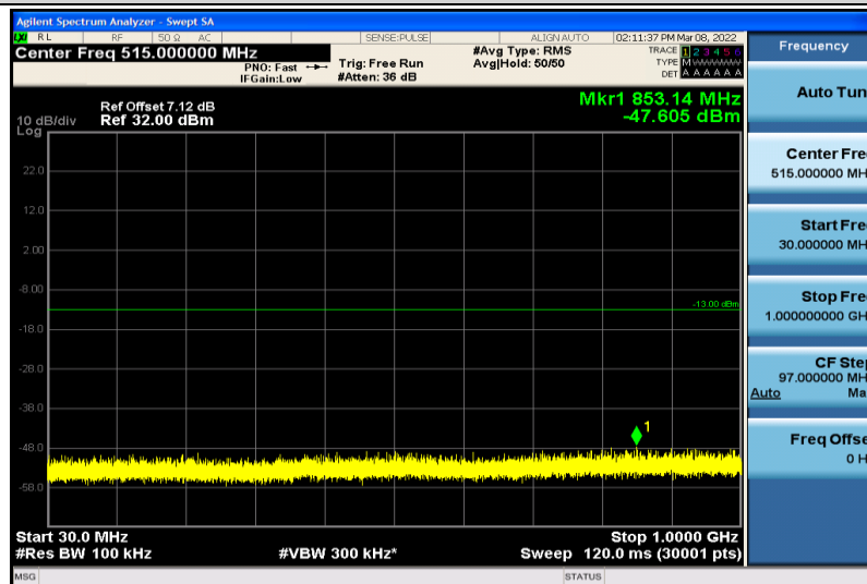
Band2-5MHz-64QAM-19175-1RB#0-30~1000MHz
