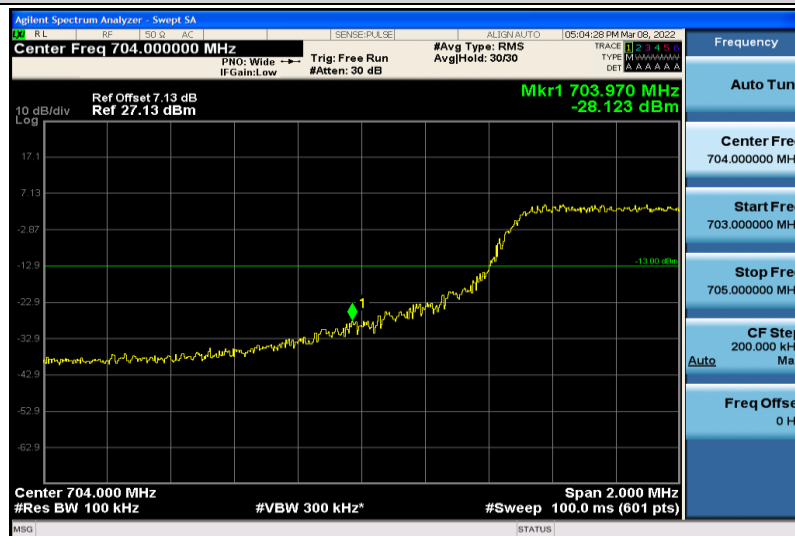
Band17-10MHz-64QAM-23780-50RB#0
