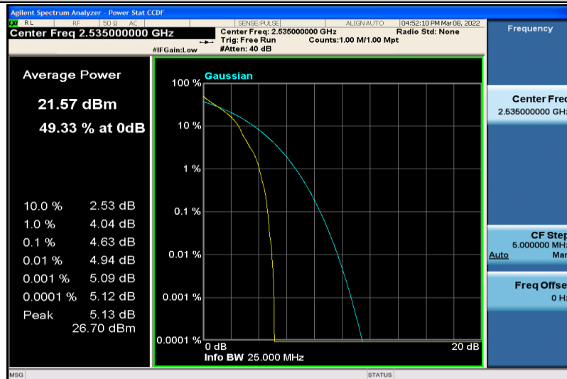
Band7-20MHz-64QAM-21100-1RB#0
