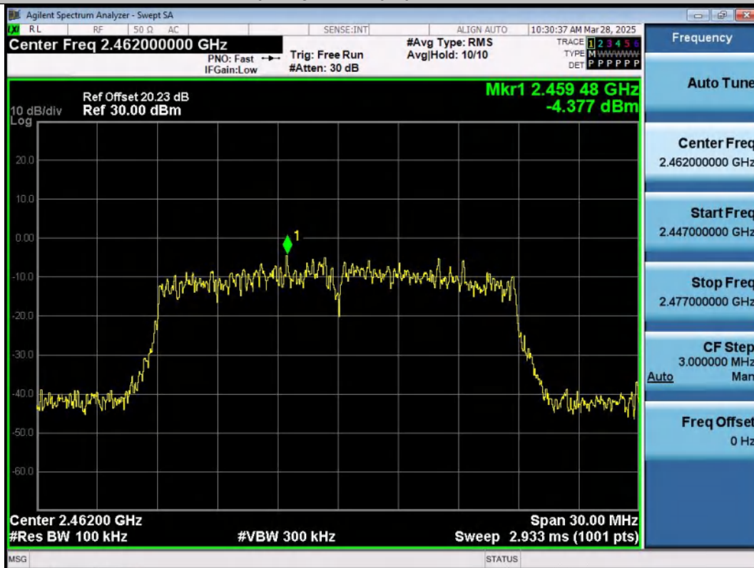
11N20MIMO-Ant2-2462-0~Reference-PASS
