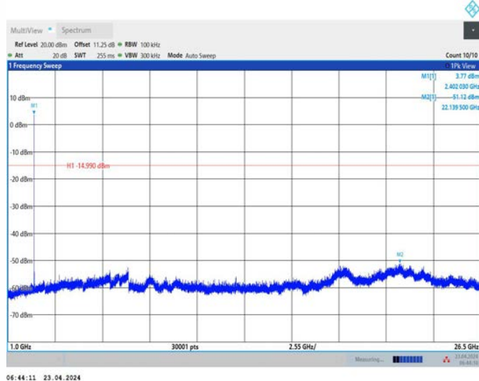
BLE_1M_Ant1_2402_1000~26500
