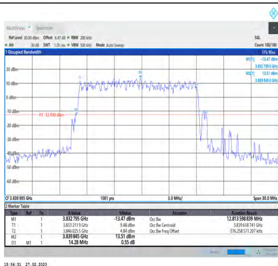
1-N77-3700-3980-30-15-M-5-DFT-256QAM-Outer_Full-36@0-Ant1-12.814-14.280-≤15-PASS
