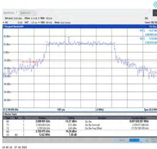
1-N77-3700-3980-30-10-L-1-DFT-QPSK-Outer_Full-2 4@0-Ant1-8.698-12.620-≤10-PASS
