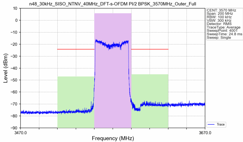
n48_30kHz_SISO_NTNV_40MHz_DFT-s-OFDM PI/2 BPSK_3570MHz_Outer_Full_Ant3
