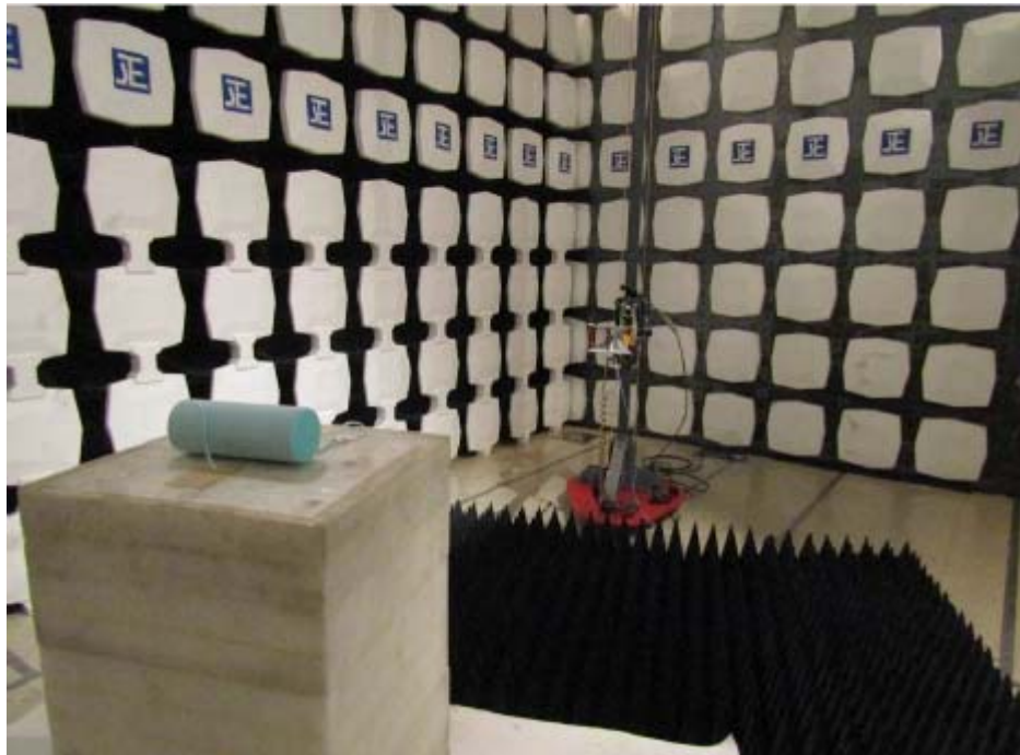
Measurement of Radiated Emission Test Set Up
