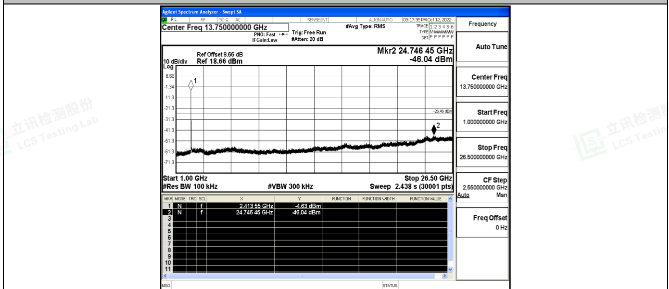
11G_Ant_2437_0~Reference
