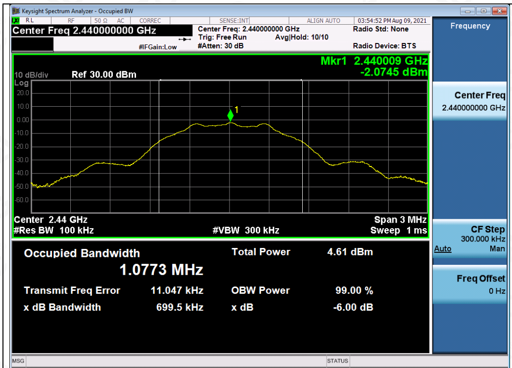
Test_Graph_LE1M_ANT1_2440_1Mbps_DTSBW
