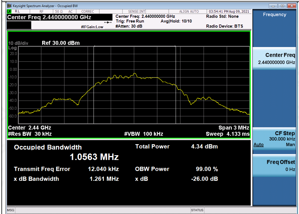
Test_Graph_LE1M_ANT1_2440_1Mbps_OBW
