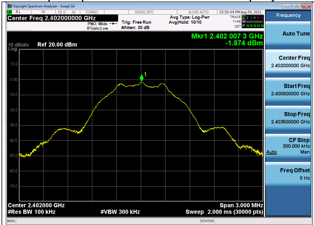
Test_Graph_LE1M_ANT1_2402_1Mbps_Reference Level
