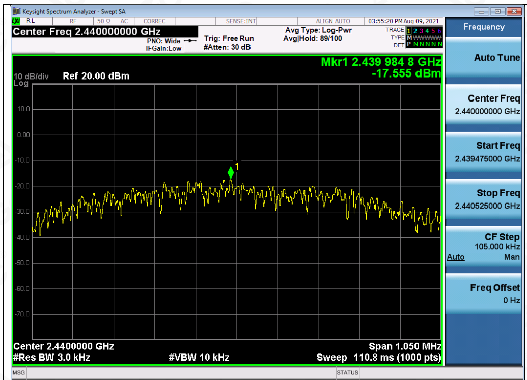
Test_Graph_LE1M_ANT1_2440_1Mbps_PSD
