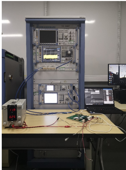
Photograph 3: Set-up photo for RF Conducted Singal test
