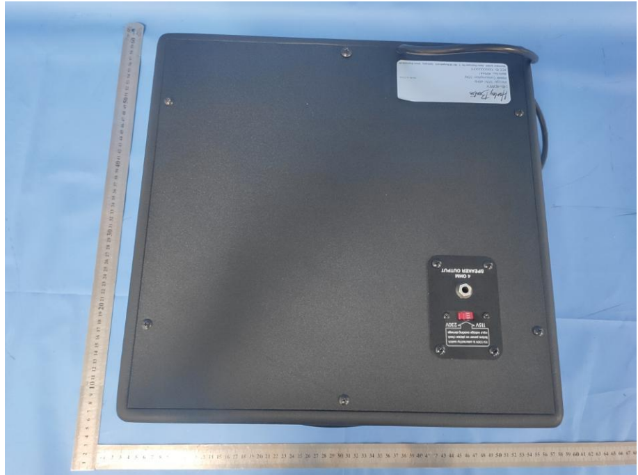
HB-40MFX with voltage selection switch
