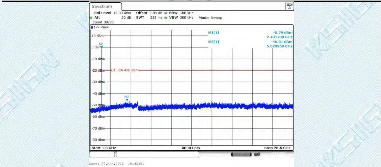
11N20SISO_Ant1_2462_1000~26500
