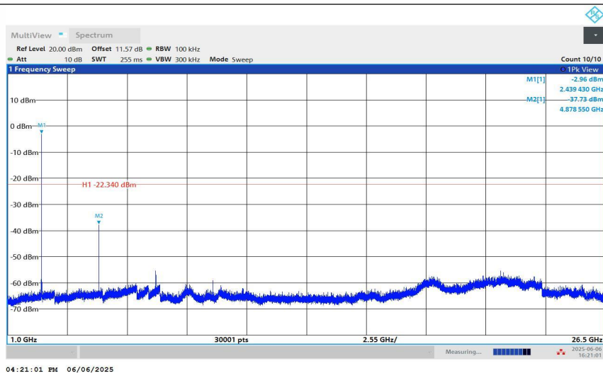
BLE_2M-Ant1-2440-1000~26500-PASS
