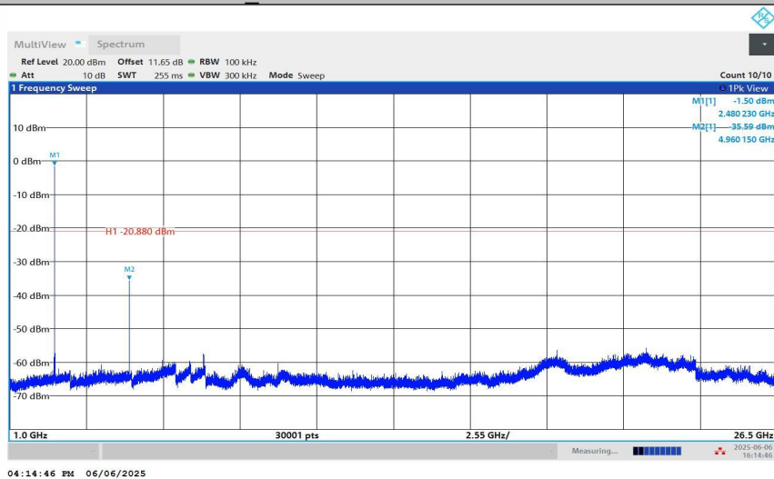
BLE_1M-Ant1-2480-1000~26500-PASS
