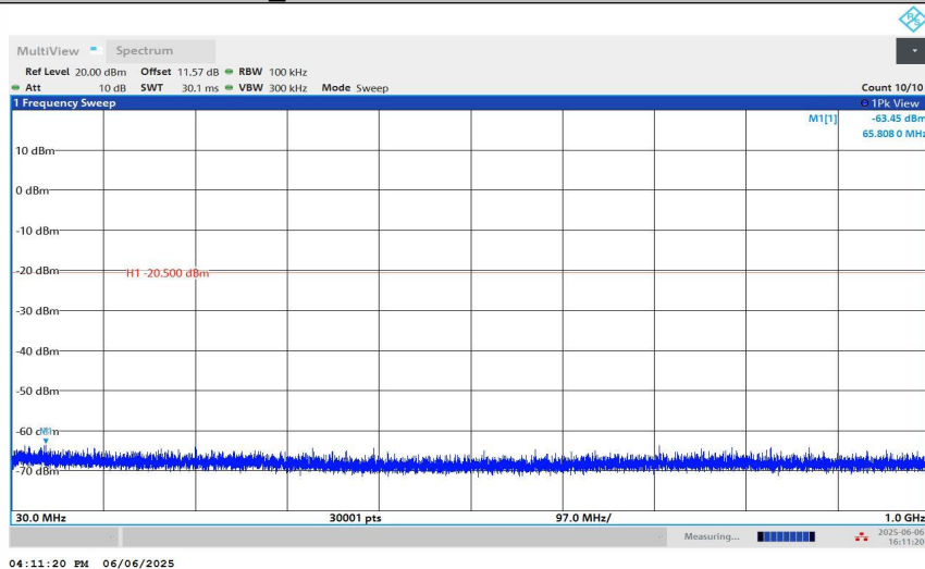
BLE_1M-Ant1-2440-30~1000-PASS
