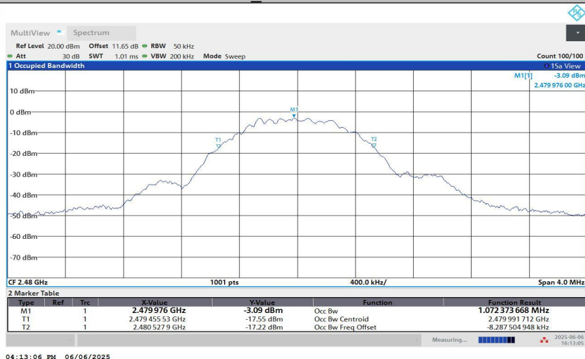
BLE_1M-Ant1-2480
