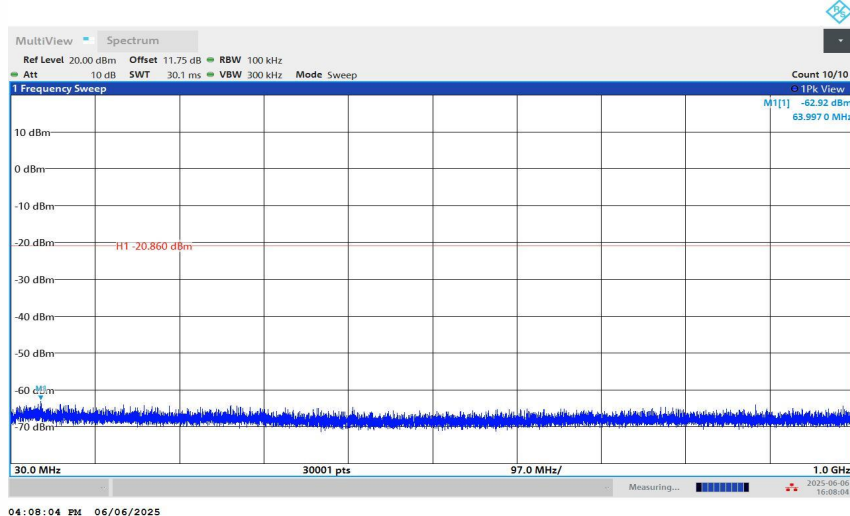
BLE_1M-Ant1-2402-30~1000-PASS
