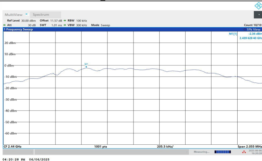
BLE_2M-Ant1-2440-PASS
