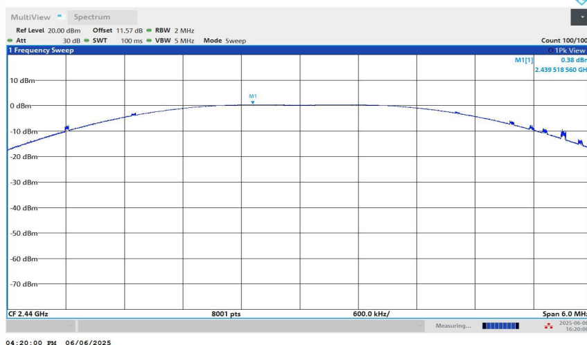
BLE_2M-Ant1-2440-PASS
