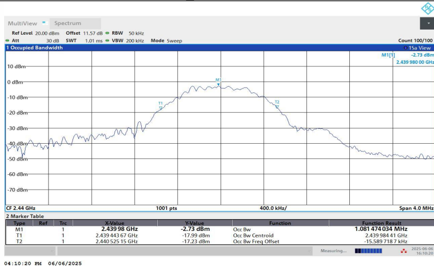
BLE_1M-Ant1-2440
