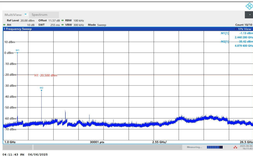
BLE_1M-Ant1-2440-1000~26500-PASS
