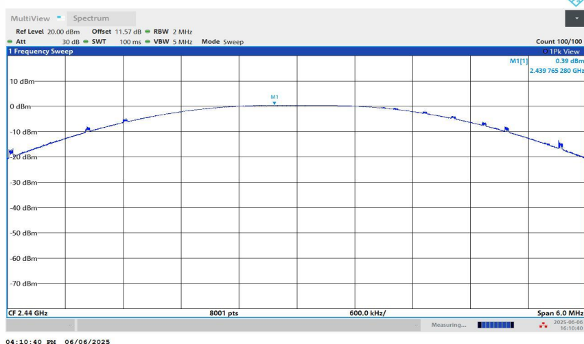
BLE_1M-Ant1-2440-PASS
