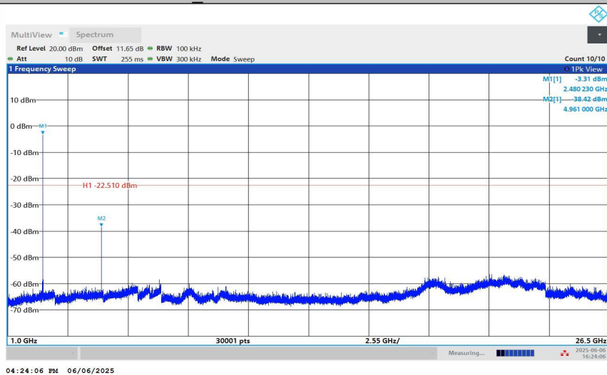
BLE_2M-Ant1-2480-1000~26500-PASS
