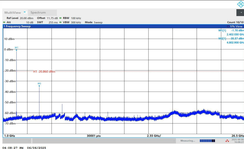
BLE_1M-Ant1-2402-1000~26500-PASS
