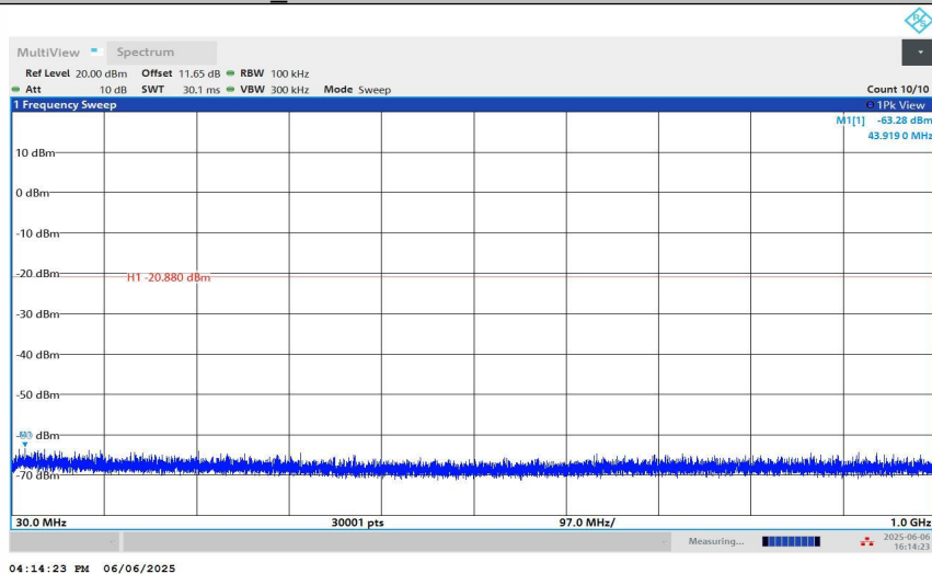
BLE_1M-Ant1-2480-30~1000-PASS
