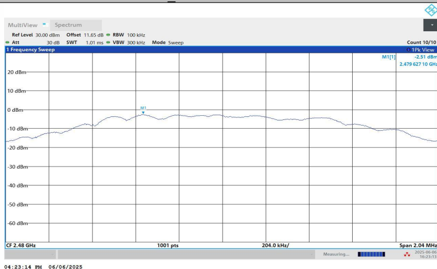
BLE_2M-Ant1-2480-PASS
