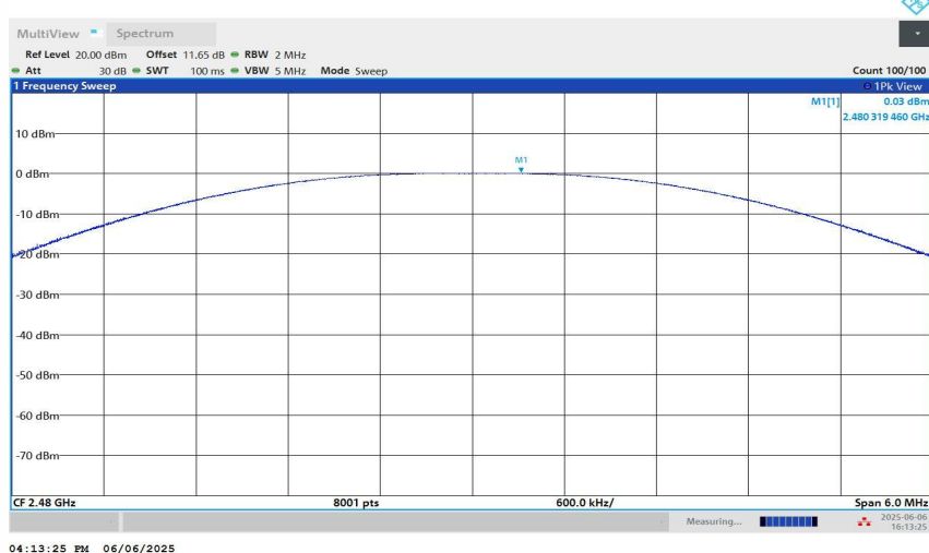
BLE_1M-Ant1-2480-PASS
