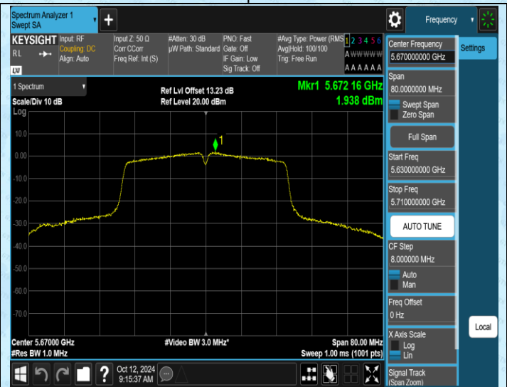
11AC40SISO-Ant2-5670-PASS
