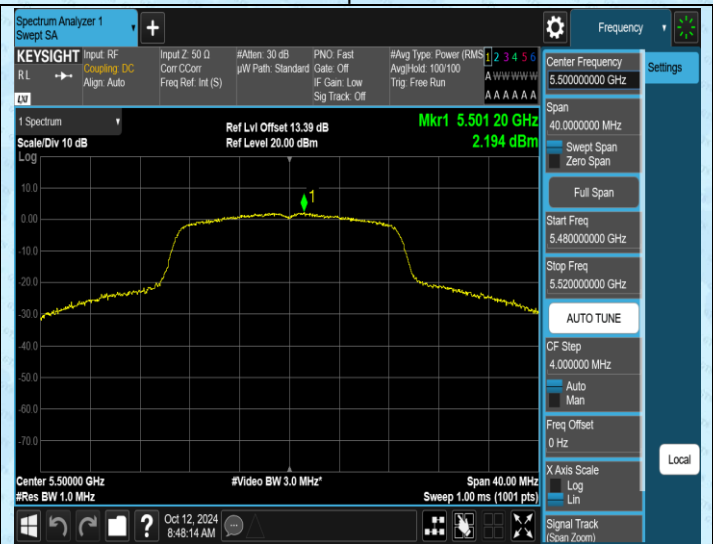
11AC20SISO-Ant2-5500-PASS
