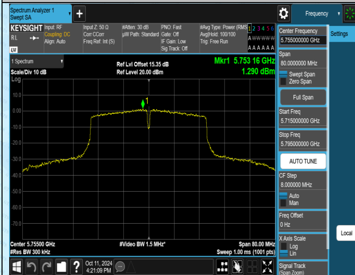
11AC40SISO-Ant1-5755-PASS
