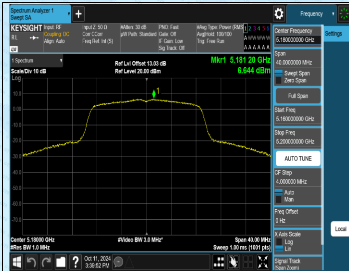
11AC20SISO-Ant1-5180-PASS
