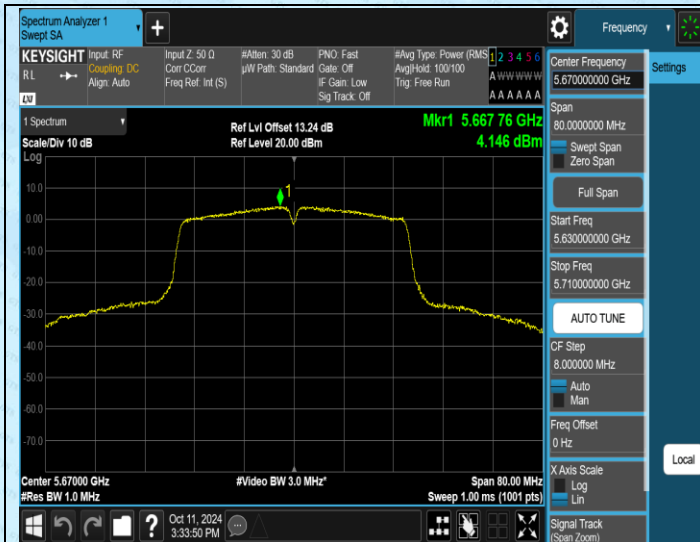
11N40SISO-Ant1-5670-PASS
