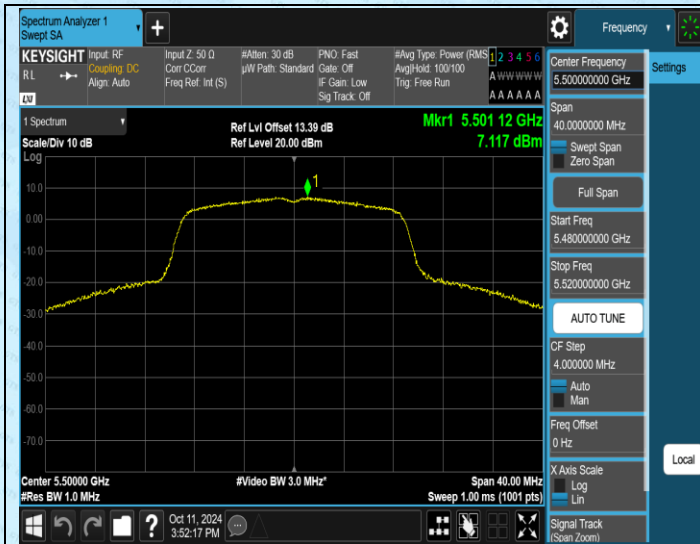
11AC20SISO-Ant1-5500-PASS
