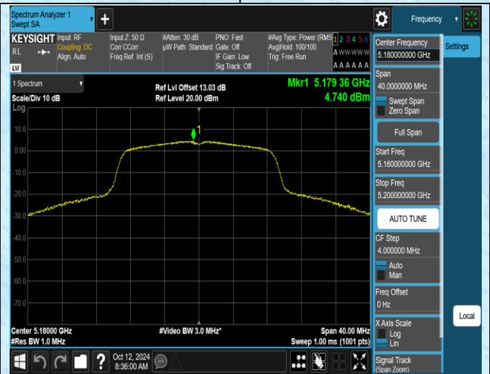
11AC20SISO-Ant2-5180-PASS
