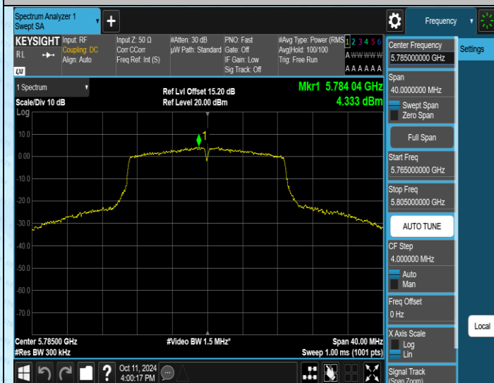
11AC20SISO-Ant1-5785-PASS
