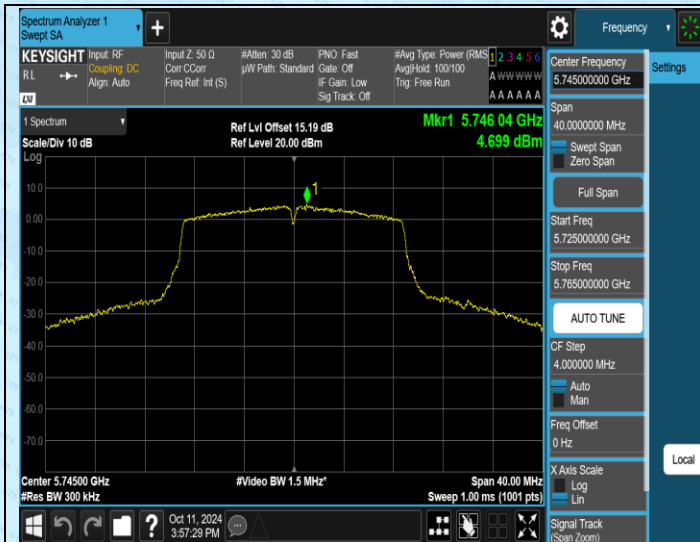
11AC20SISO-Ant1-5745-PASS
