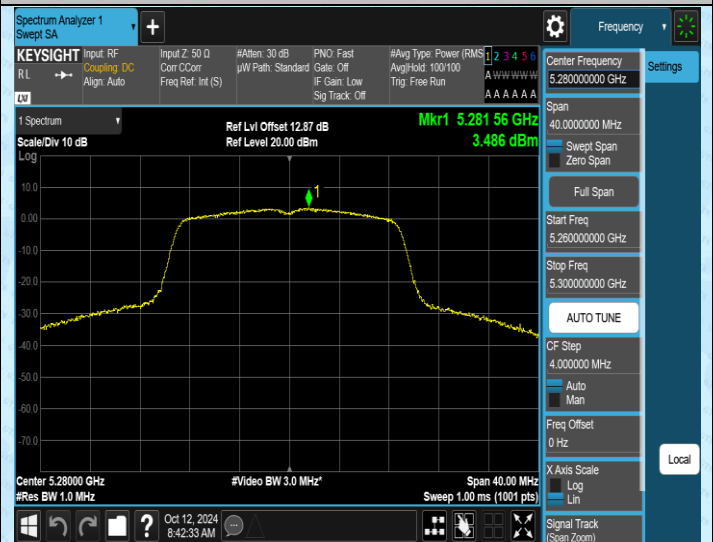
11AC20SISO-Ant2-5280-PASS
