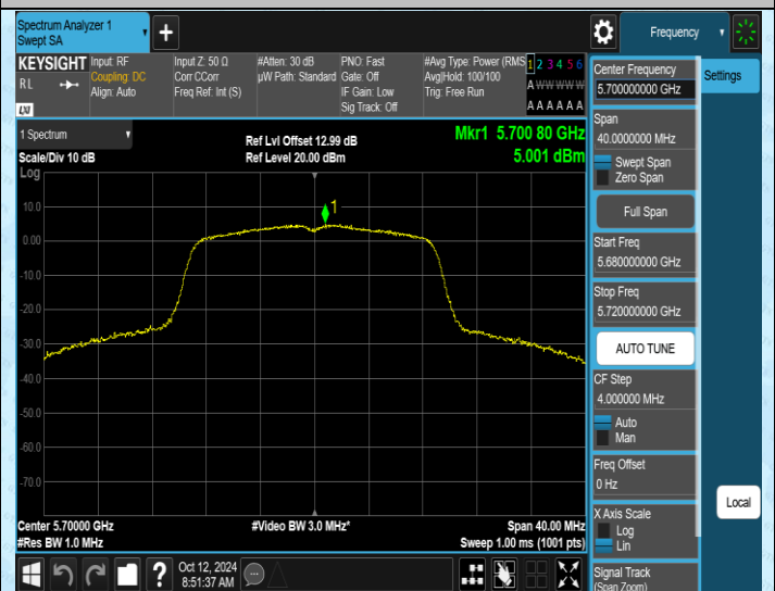
11AC20SISO-Ant2-5700-PASS
