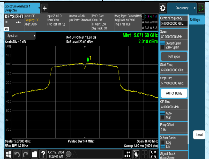
11N40SISO-Ant2-5670-PASS
