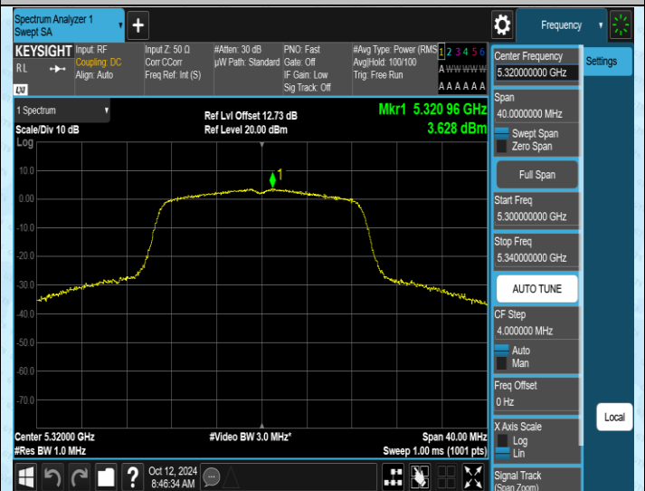
11AC20SISO-Ant2-5320-PASS
