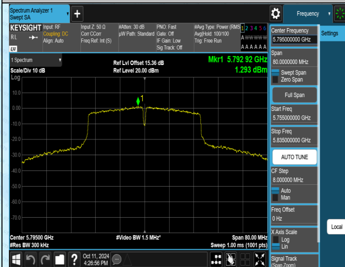
11AC40SISO-Ant1-5795-PASS
