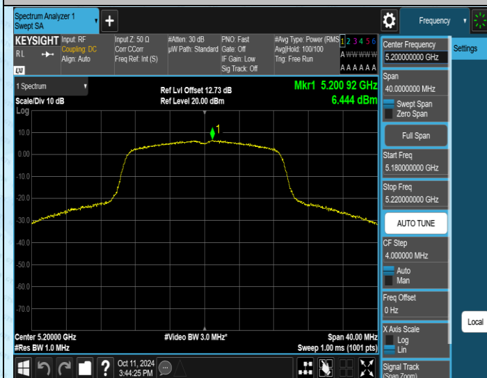
11AC20SISO-Ant1-5200-PASS
