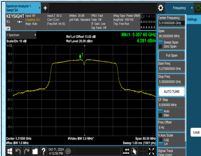
11AC40SISO-Ant1-5310-PASS
