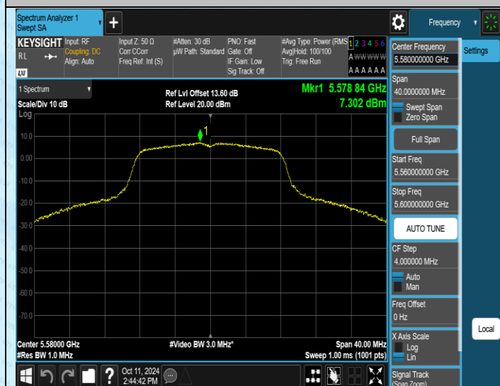
11A-Ant1-5580-PASS
