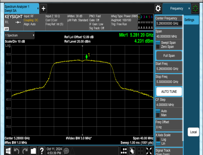
11A-Ant2-5280-PASS
