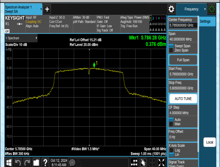
11N20SISO-Ant2-5785-PASS
