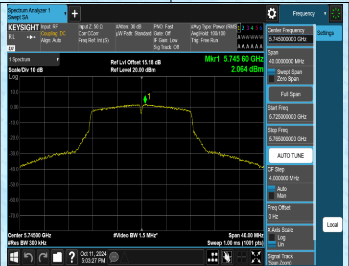
11A-Ant2-5745-PASS
