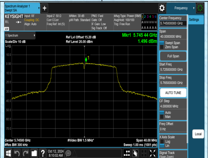
11N20SISO-Ant2-5745-PASS
