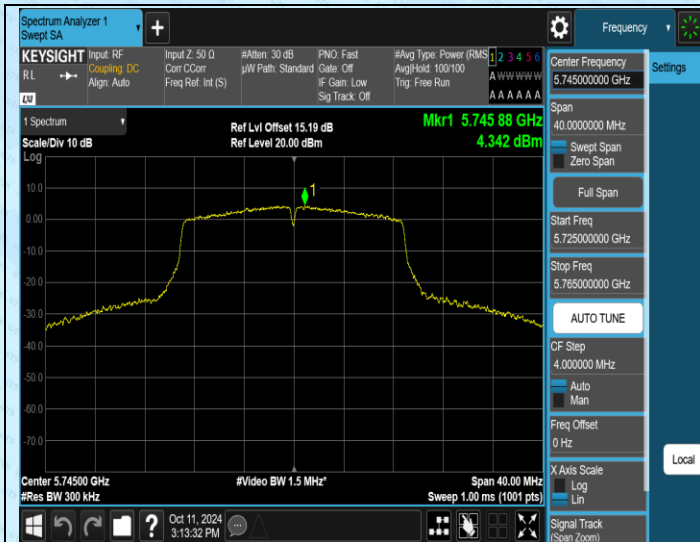
11N20SISO-Ant1-5745-PASS
