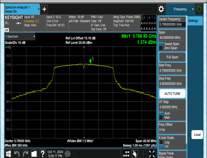
11A-Ant2-5785-PASS
