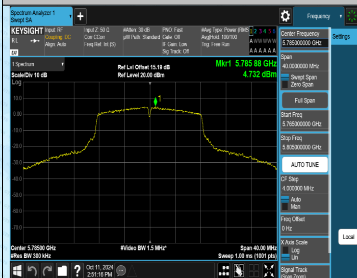
11A-Ant1-5785-PASS
