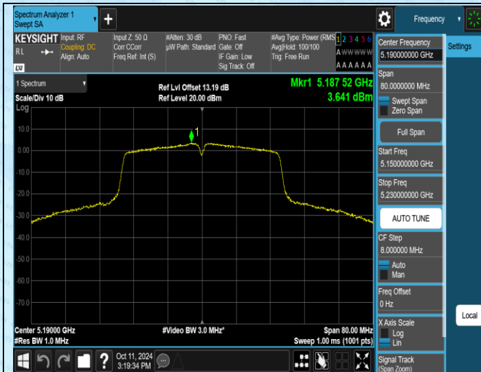
11N40SISO-Ant1-5190-PASS
