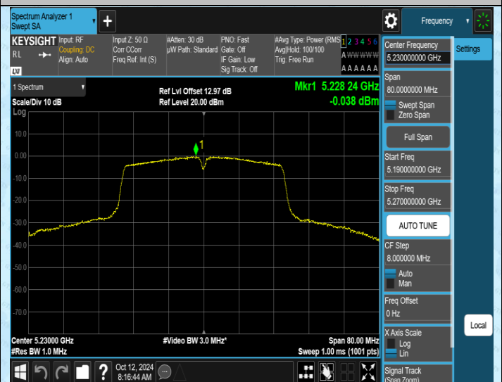
11N40SISO-Ant2-5230-PASS
