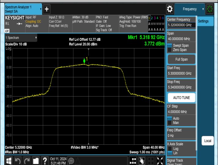
11N20SISO-Ant2-5320-PASS
