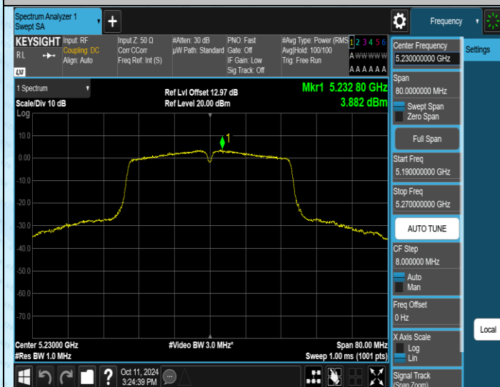
11N40SISO-Ant1-5230-PASS
