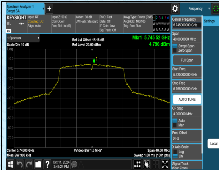
11A-Ant1-5745-PASS
