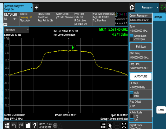
11A-Ant2-5580-PASS
