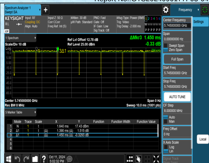
NTNV-11A-Ant2-5745
