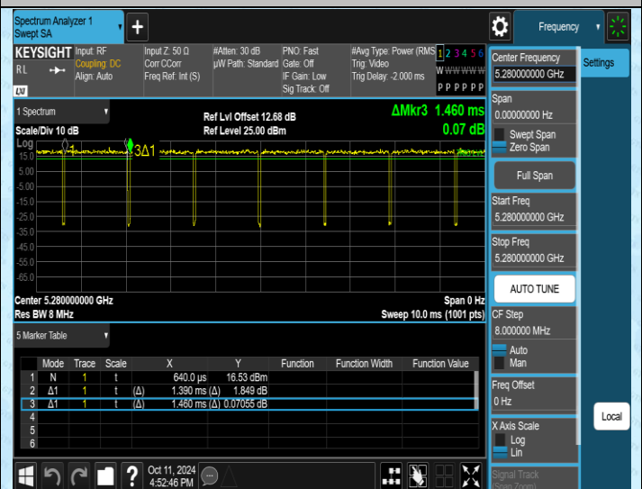
NTNV-11A-Ant2-5280
