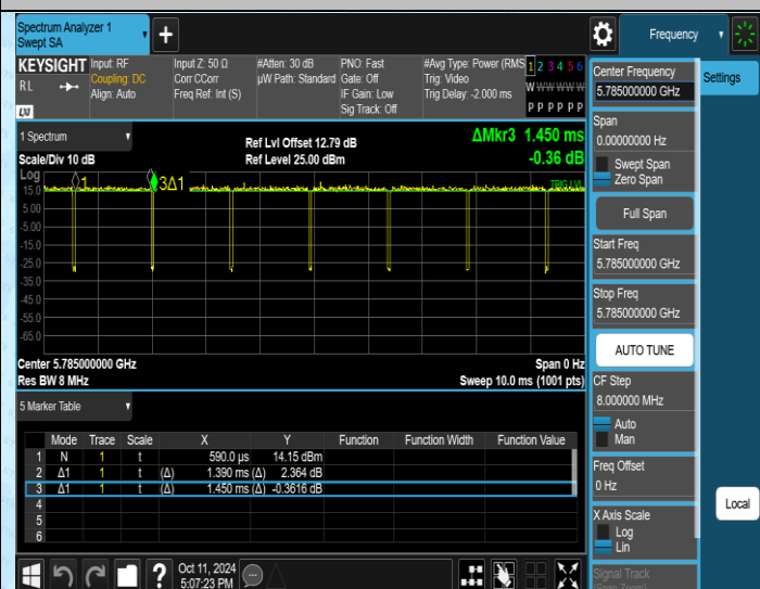
NTNV-11A-Ant2-5785
