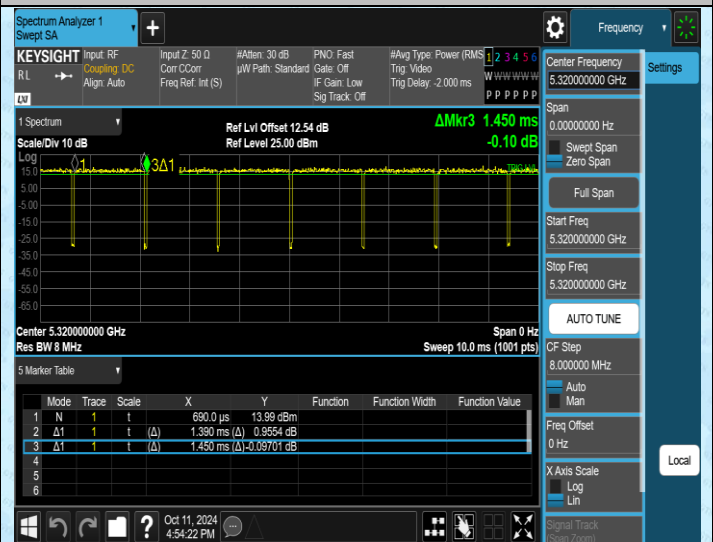
NTNV-11A-Ant2-5320
