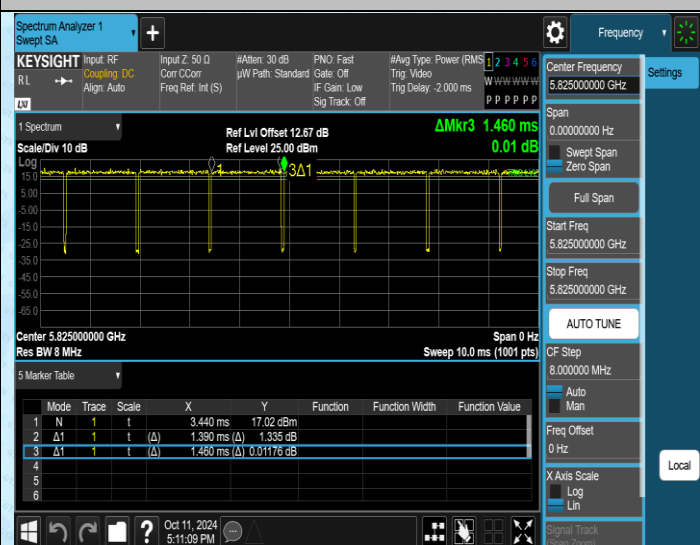
NTNV-11A-Ant2-5825
