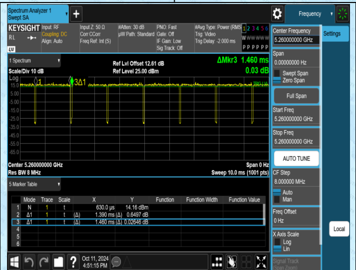
NTNV-11A-Ant2-5260
