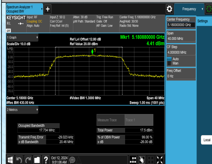
11N20MIMO-Ant1-5180
