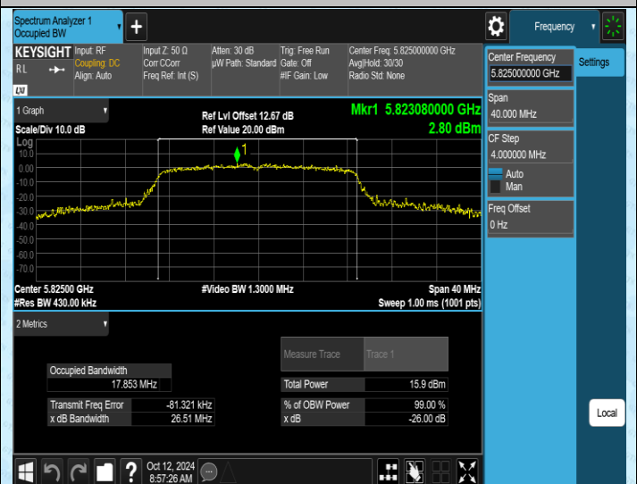
11AC20SISO-Ant2-5825
