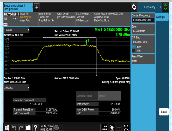
11N20MIMO-Ant2-5180
