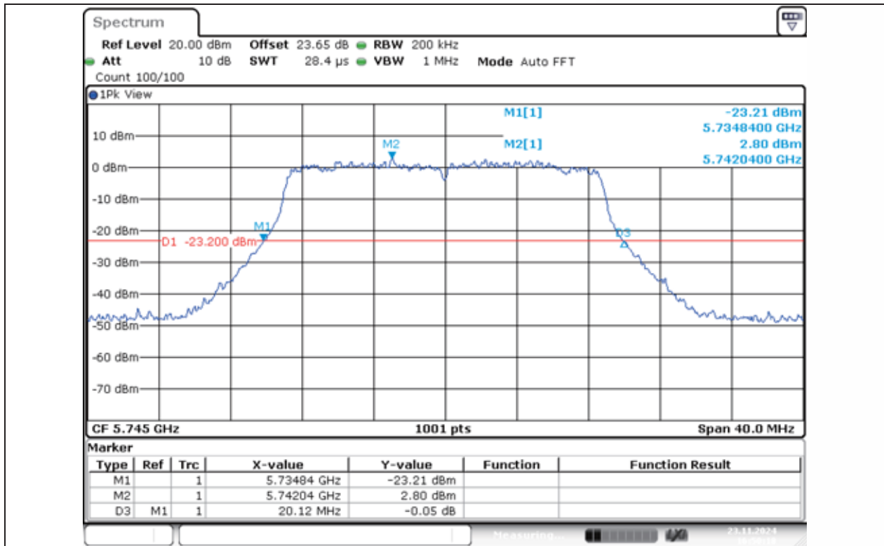
11AC20MIMO-Ant1-5745
