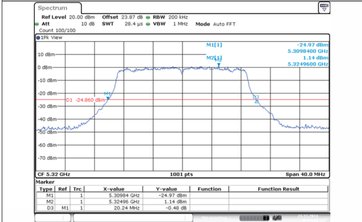
11AC20MIMO-Ant1-5320
