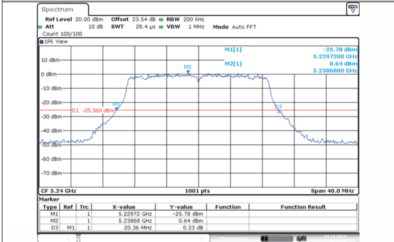
11AC20MIMO-Ant1-5240
