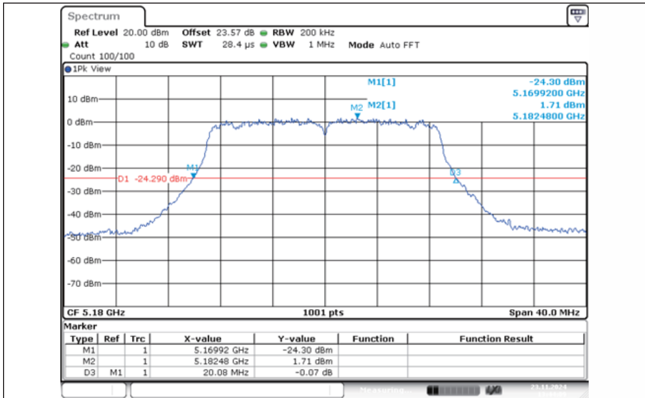
11N20MIMO-Ant1-5180
