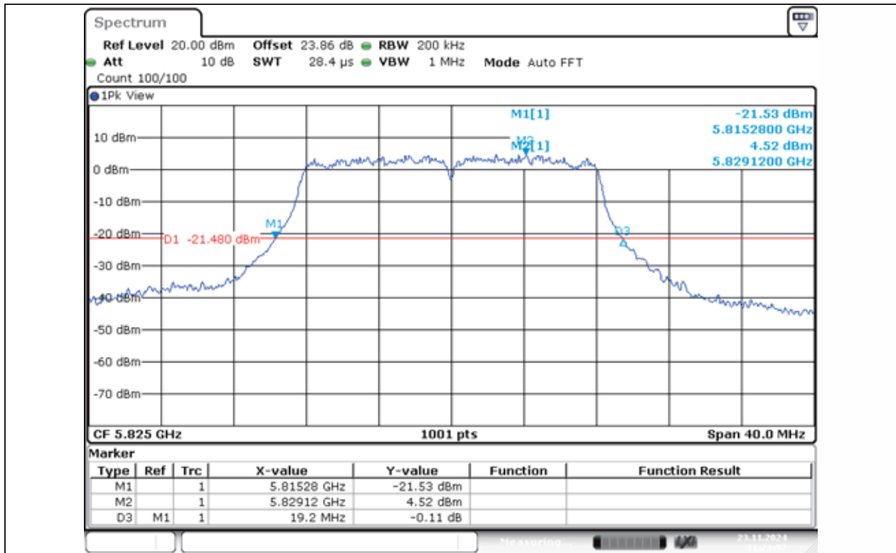
11A-Ant1-5825
