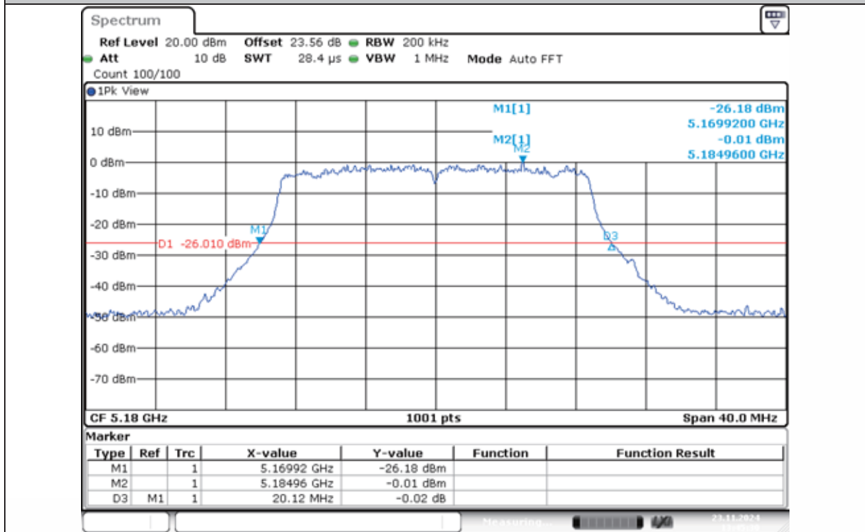
11N20MIMO-Ant1-5180
