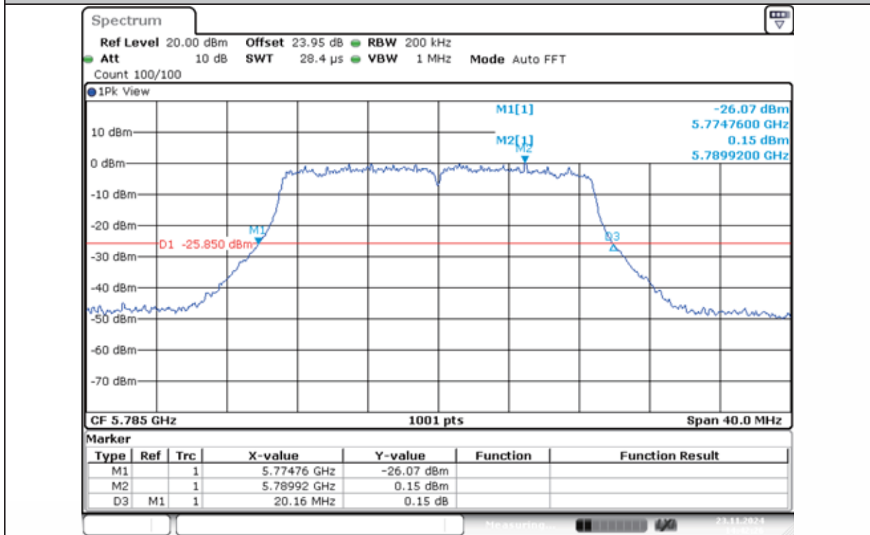
11N20MIMO-Ant1-5785
