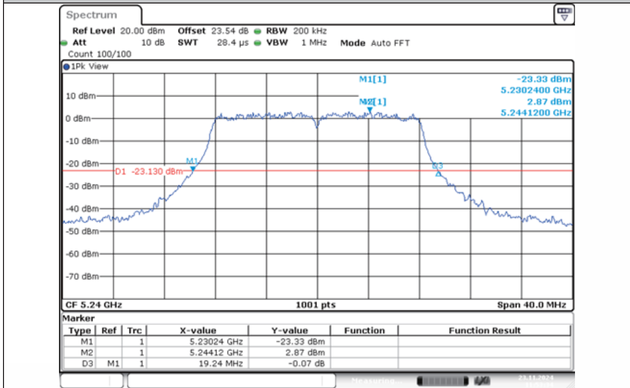
11A-Ant1-5240
