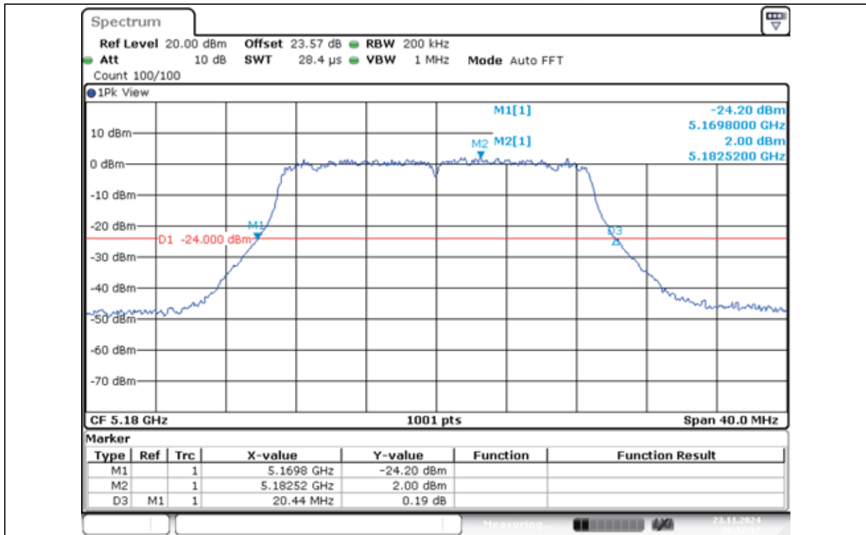
11AC20MIMO-Ant1-5180
