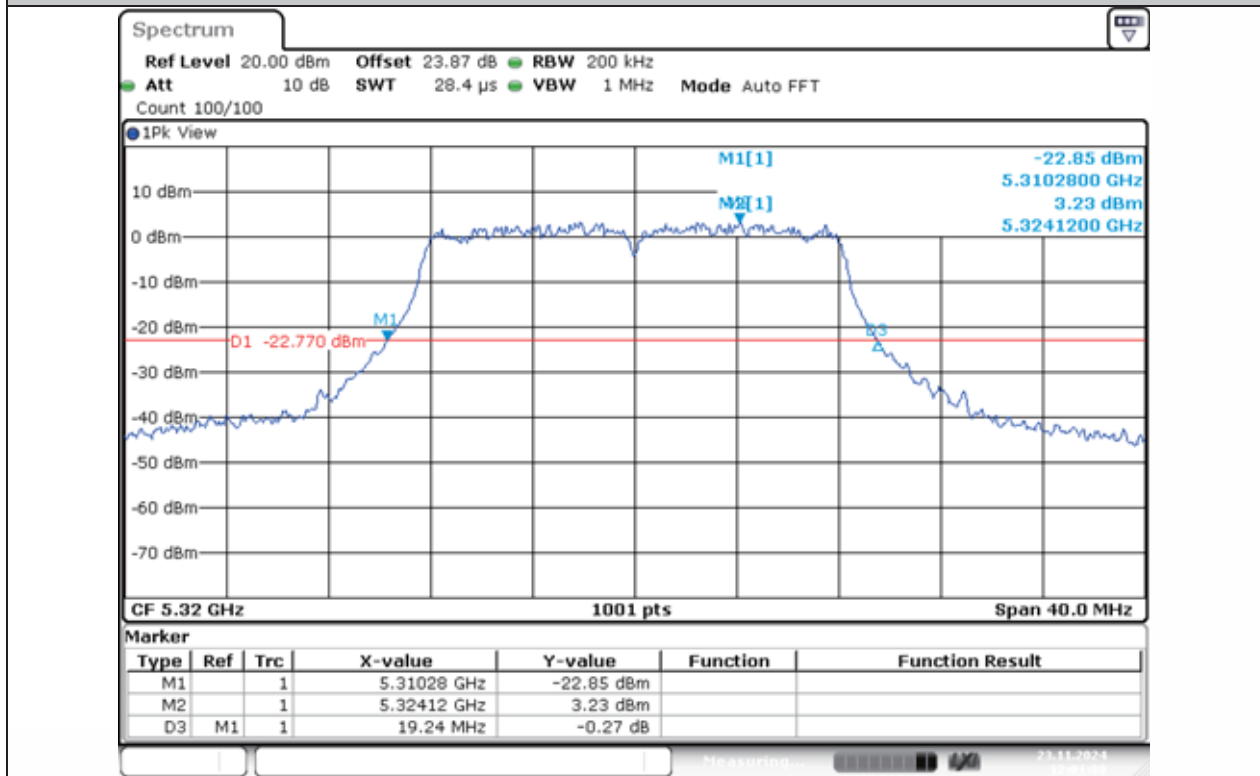
11A-Ant1-5320
