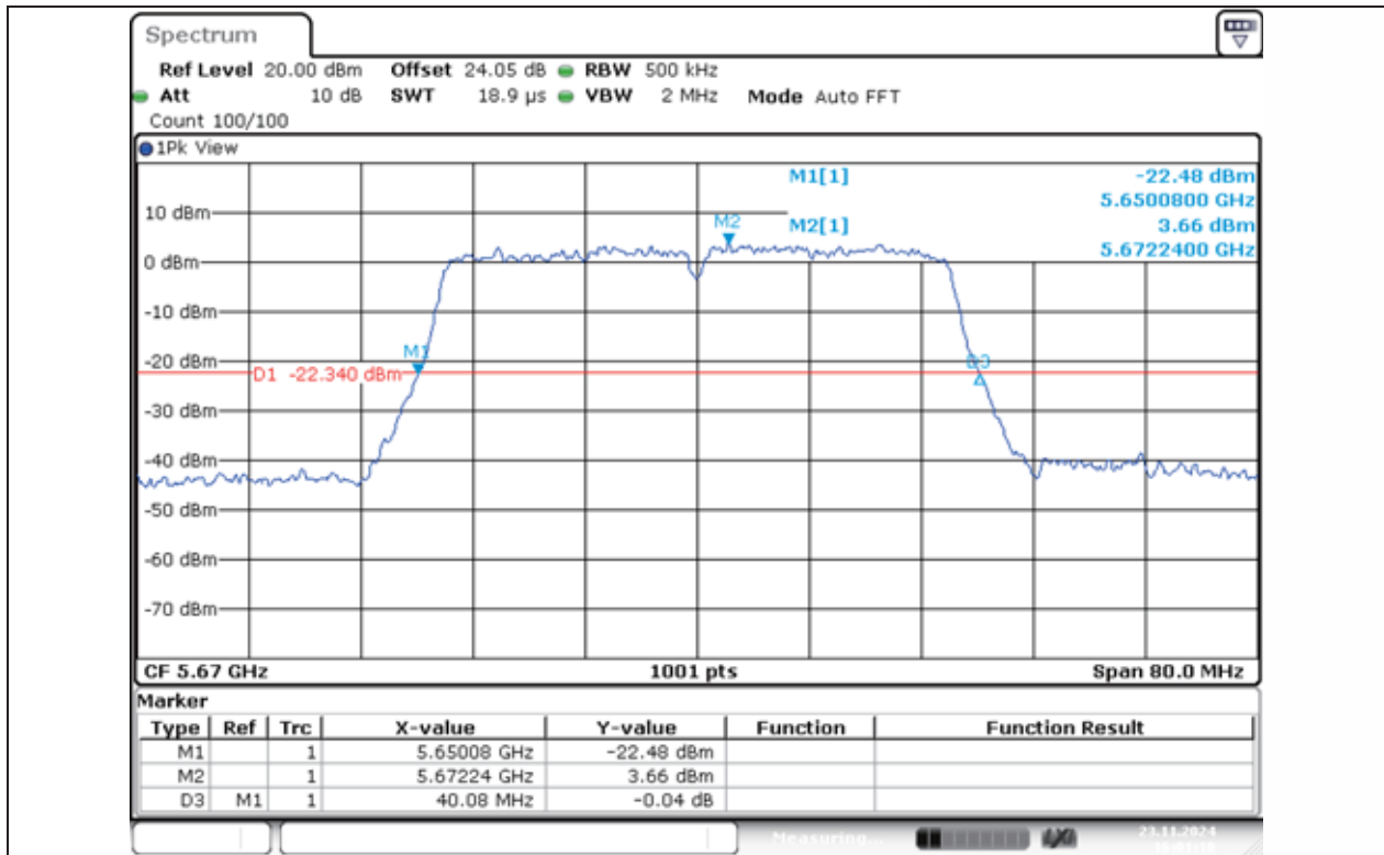
11N40MIMO-Ant1-5670
