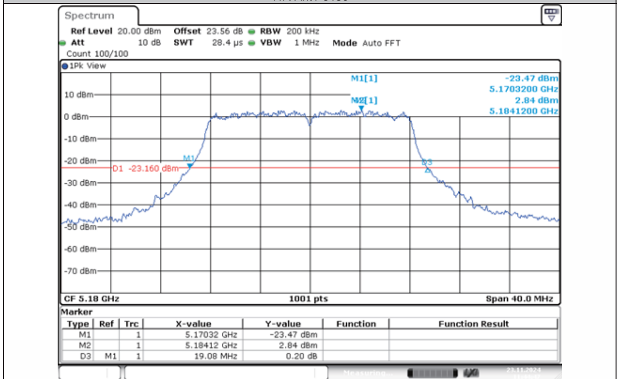
11A-Ant1-5180
