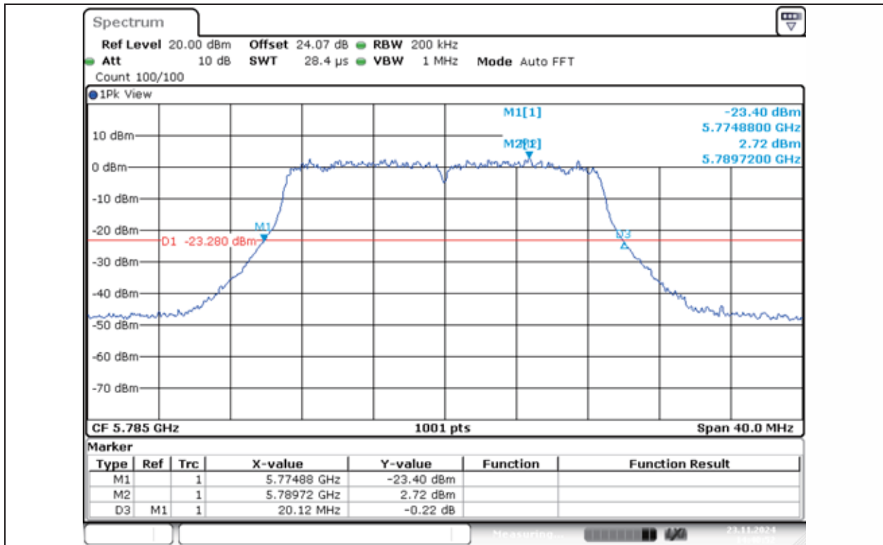
11N20MIMO-Ant1-5785
