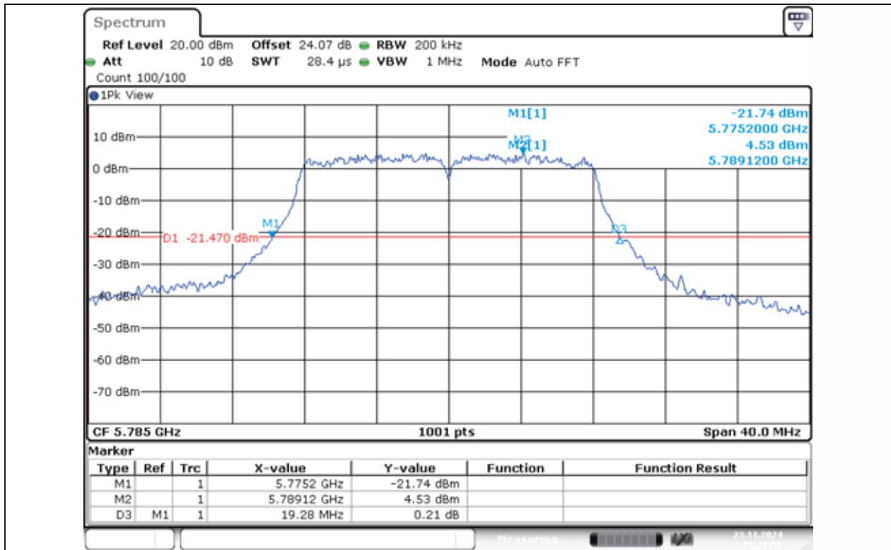
11A-Ant1-5785
