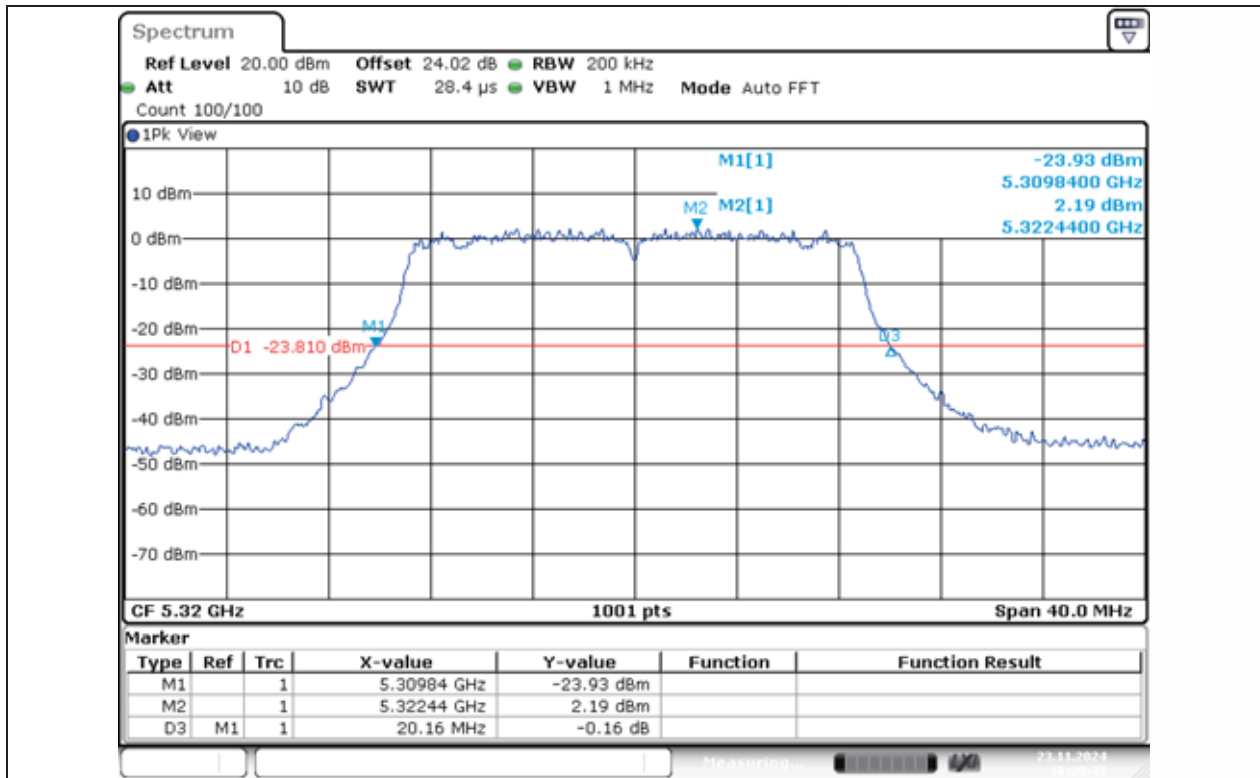
11AC20MIMO-Ant1-5320
