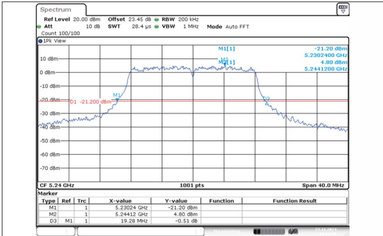
11A-Ant1-5240
