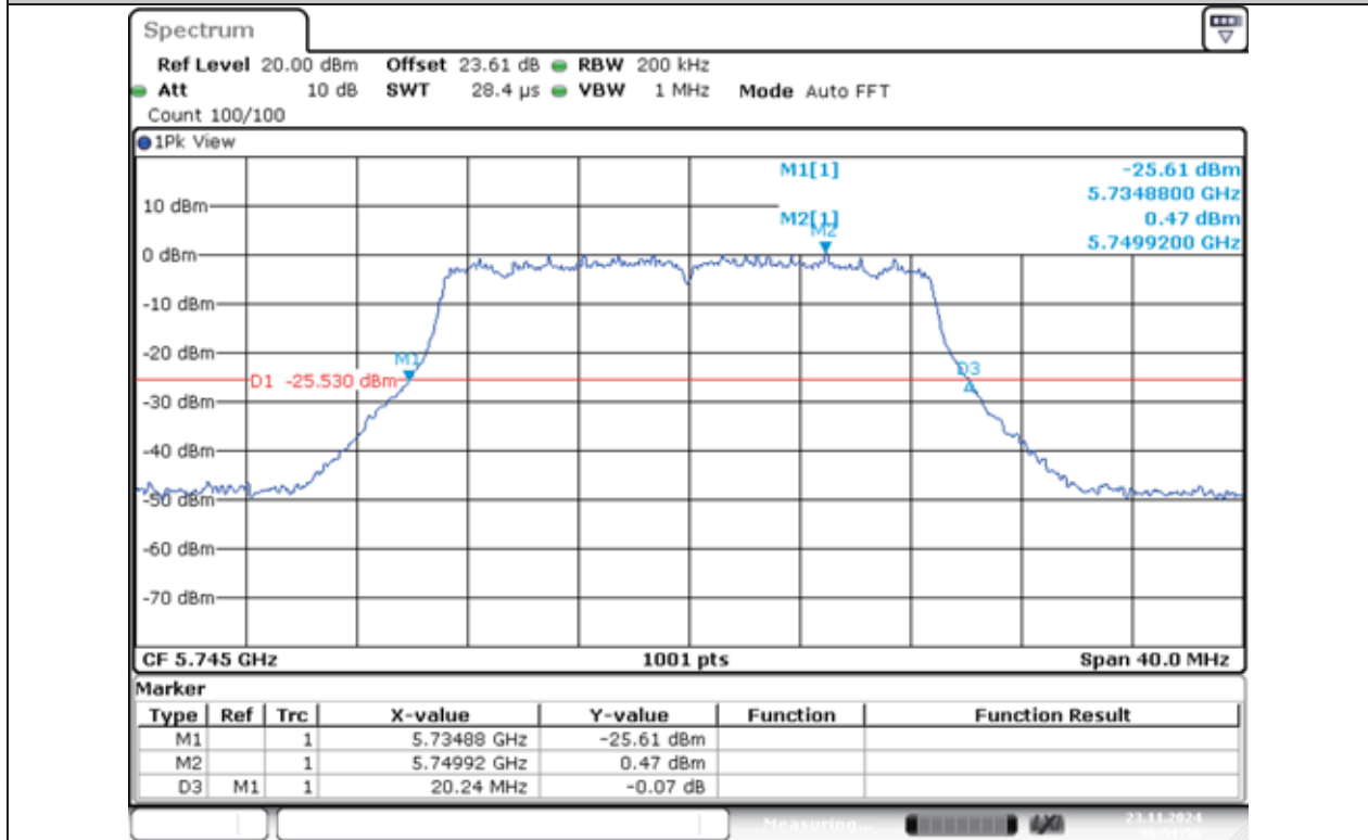
11AC20MIMO-Ant1-5745
