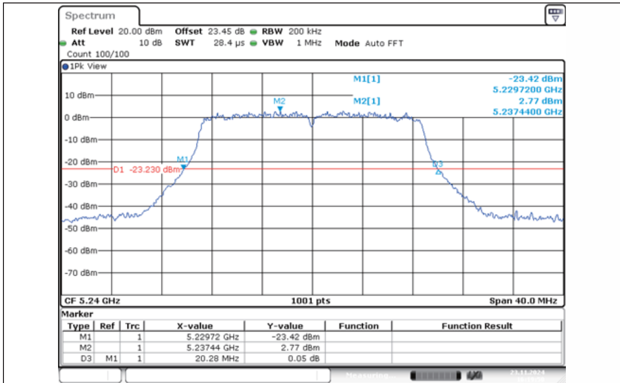
11AC20MIMO-Ant1-5240
