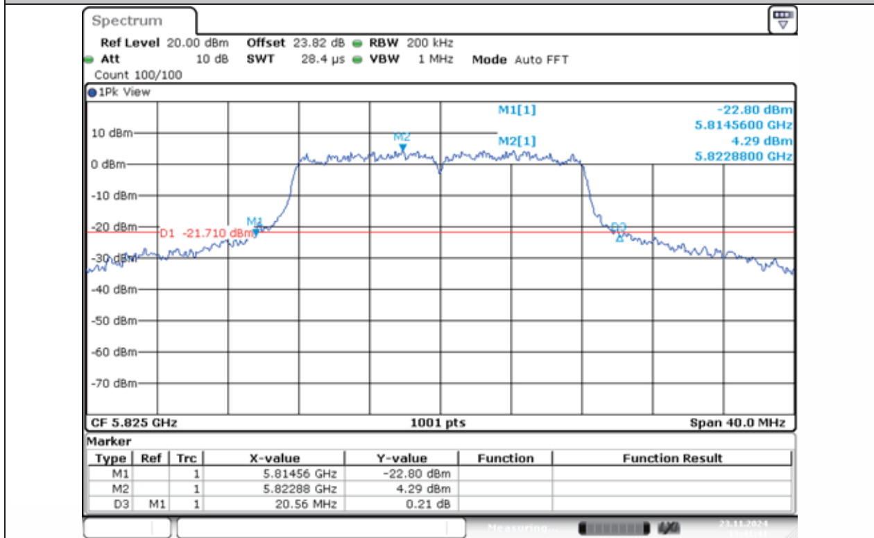
11A-Ant1-5825
