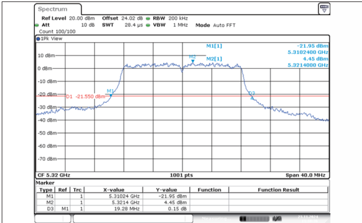
11A-Ant1-5320
