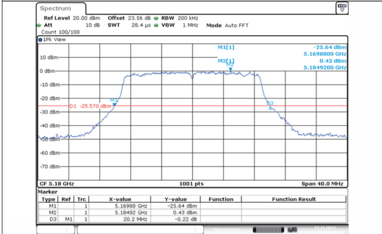
11AC20MIMO-Ant1-5180
