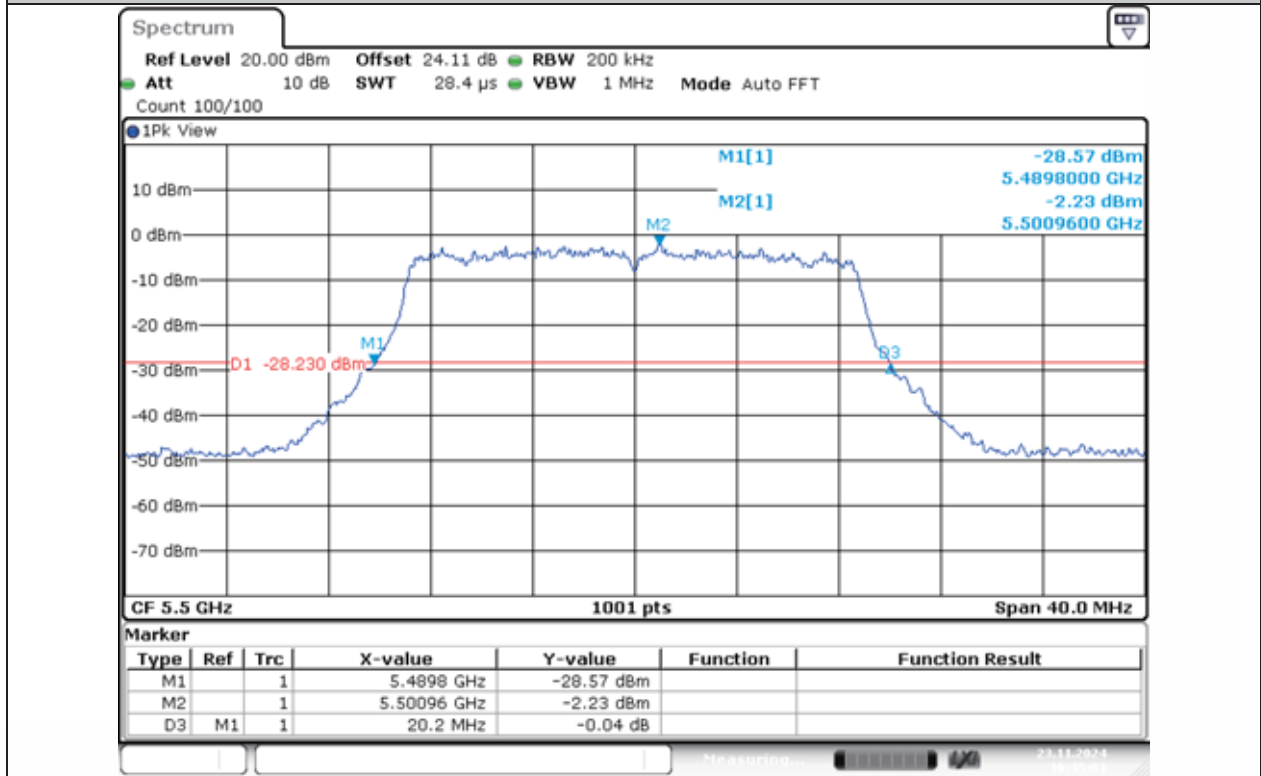
11AC20MIMO-Ant1-5500
