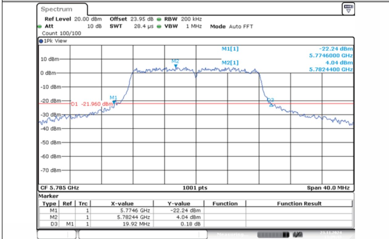
11A-Ant1-5785
