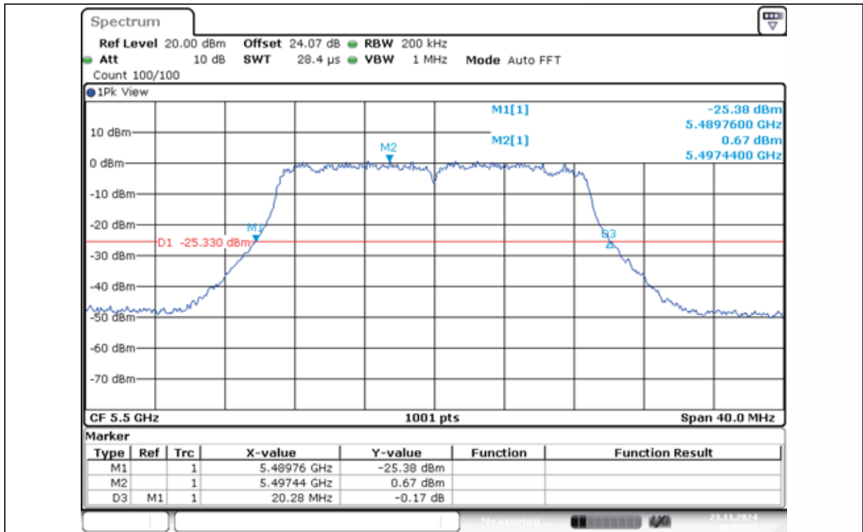
11AC20MIMO-Ant1-5500
