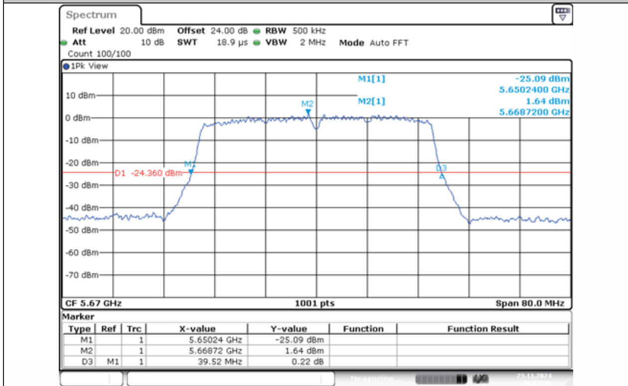
11N40MIMO-Ant1-5670
