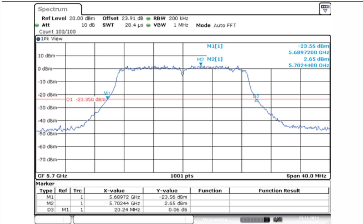
11AC20MIMO-Ant1-5700
