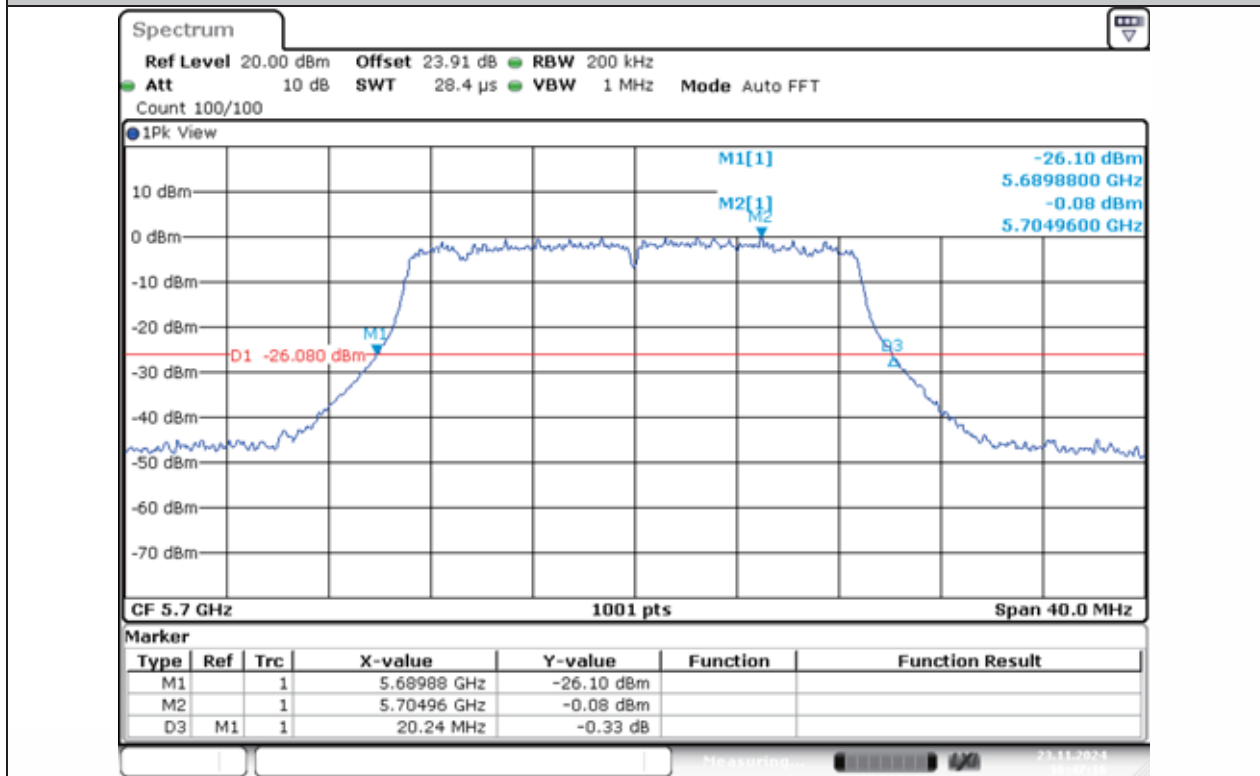
11AC20MIMO-Ant1-5700
